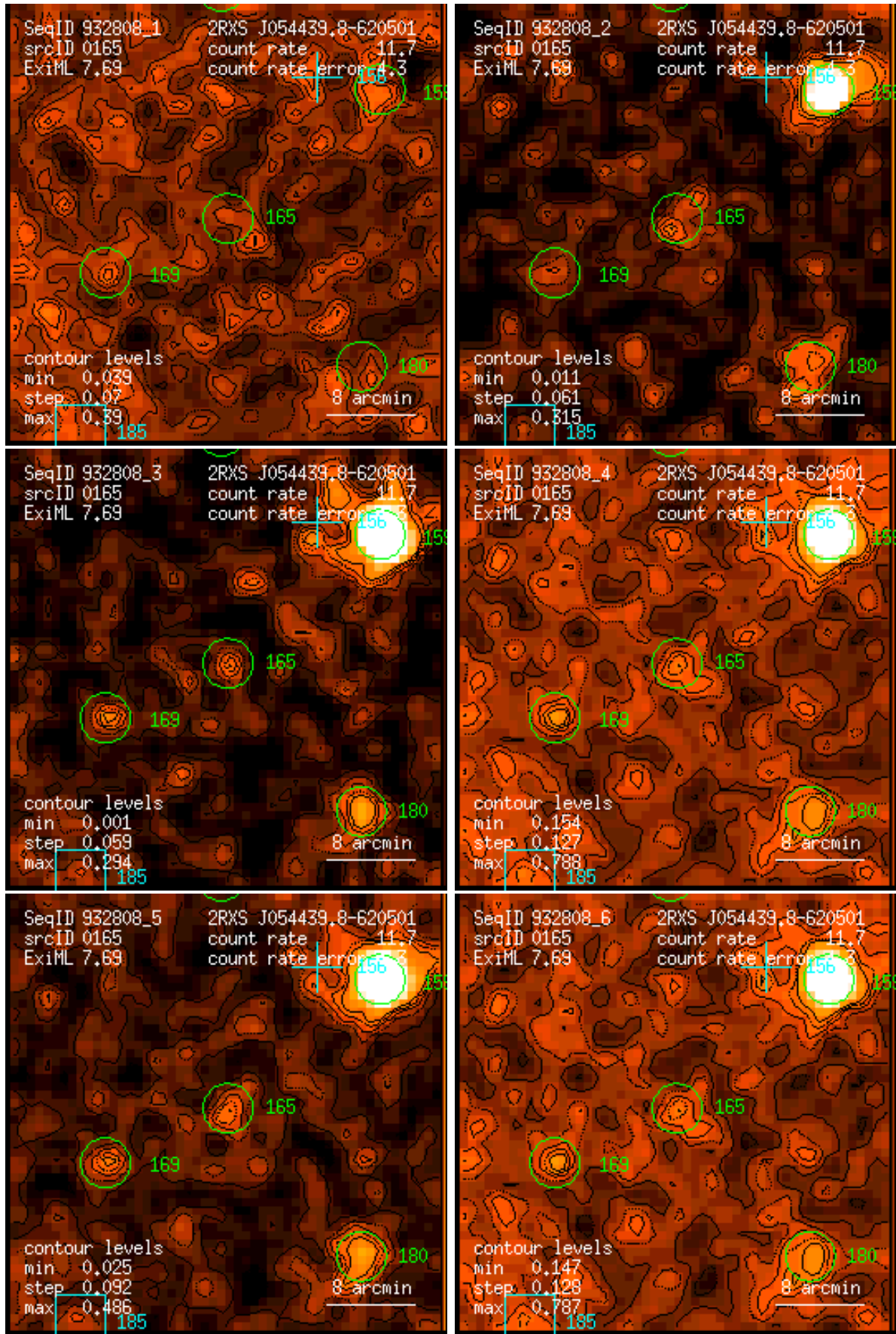
Figure 165: RASS 932808: detection 0165: band rate images, Gaussian filter: (1) PSPC channels 11 – 41, (2) 52 – 90, (3) 91 – 201, (4) 11 – 235, (5) 52 – 201, (6) 11 – 201. Broad band rates in counts/ks. Band rate contour levels in counts/ks/arcmin 2 .
