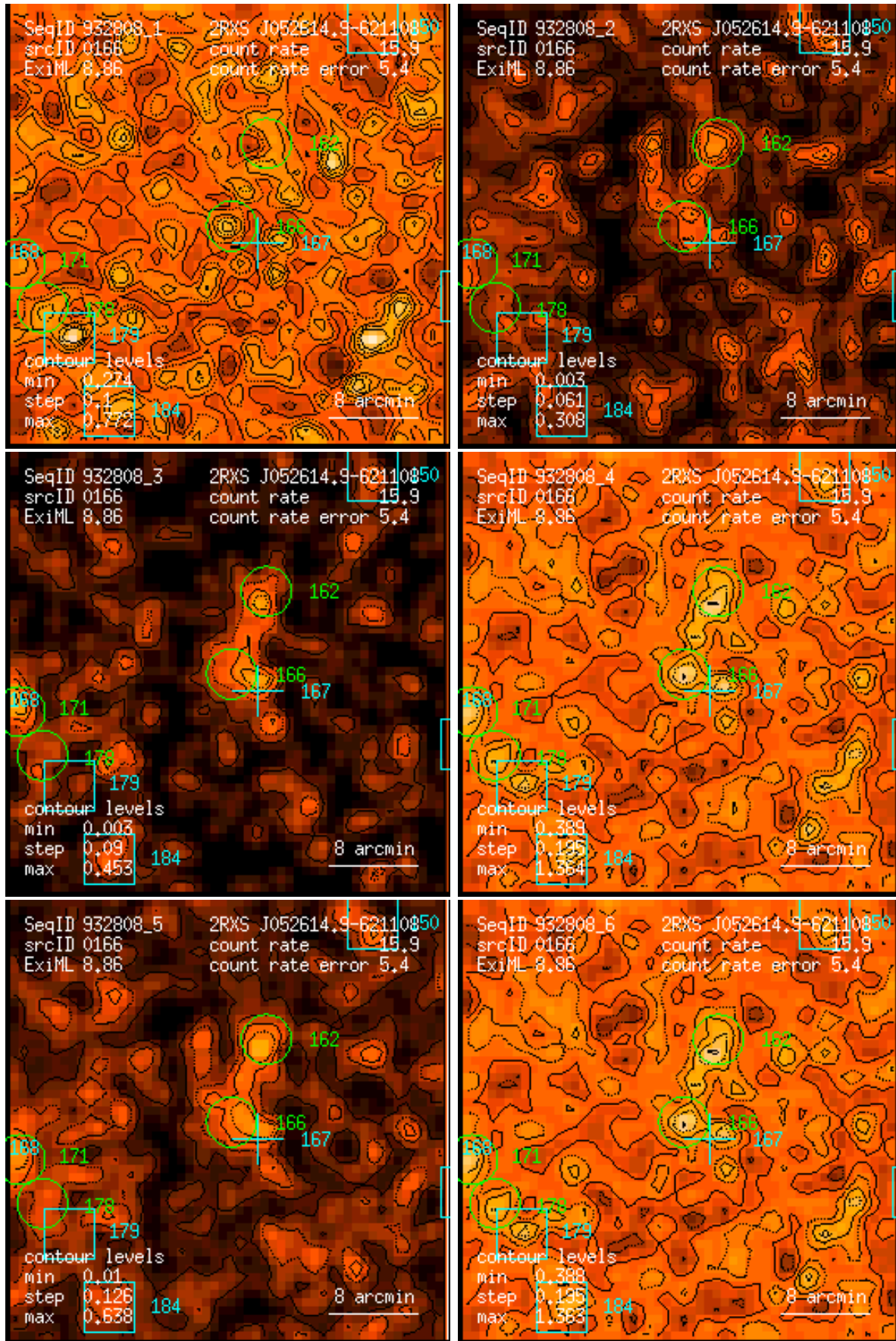
Figure 166: RASS 932808: detection 0166: band rate images, Gaussian filter: (1) PSPC channels 11 – 41, (2) 52 – 90, (3) 91 – 201, (4) 11 – 235, (5) 52 – 201, (6) 11 – 201. Broad band rates in counts/ks. Band rate contour levels in counts/ks/arcmin 2 .
