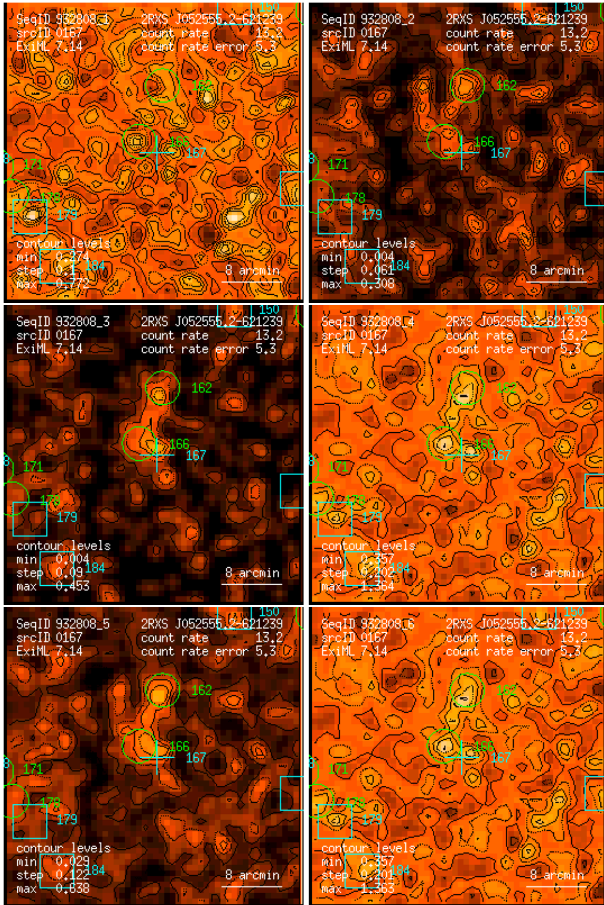
Figure 167: RASS 932808: detection 0167: band rate images, Gaussian filter: (1) PSPC channels 11 – 41, (2) 52 – 90, (3) 91 – 201, (4) 11 – 235, (5) 52 – 201, (6) 11 – 201. Broad band rates in counts/ks. Band rate contour levels in counts/ks/arcmin 2 .
