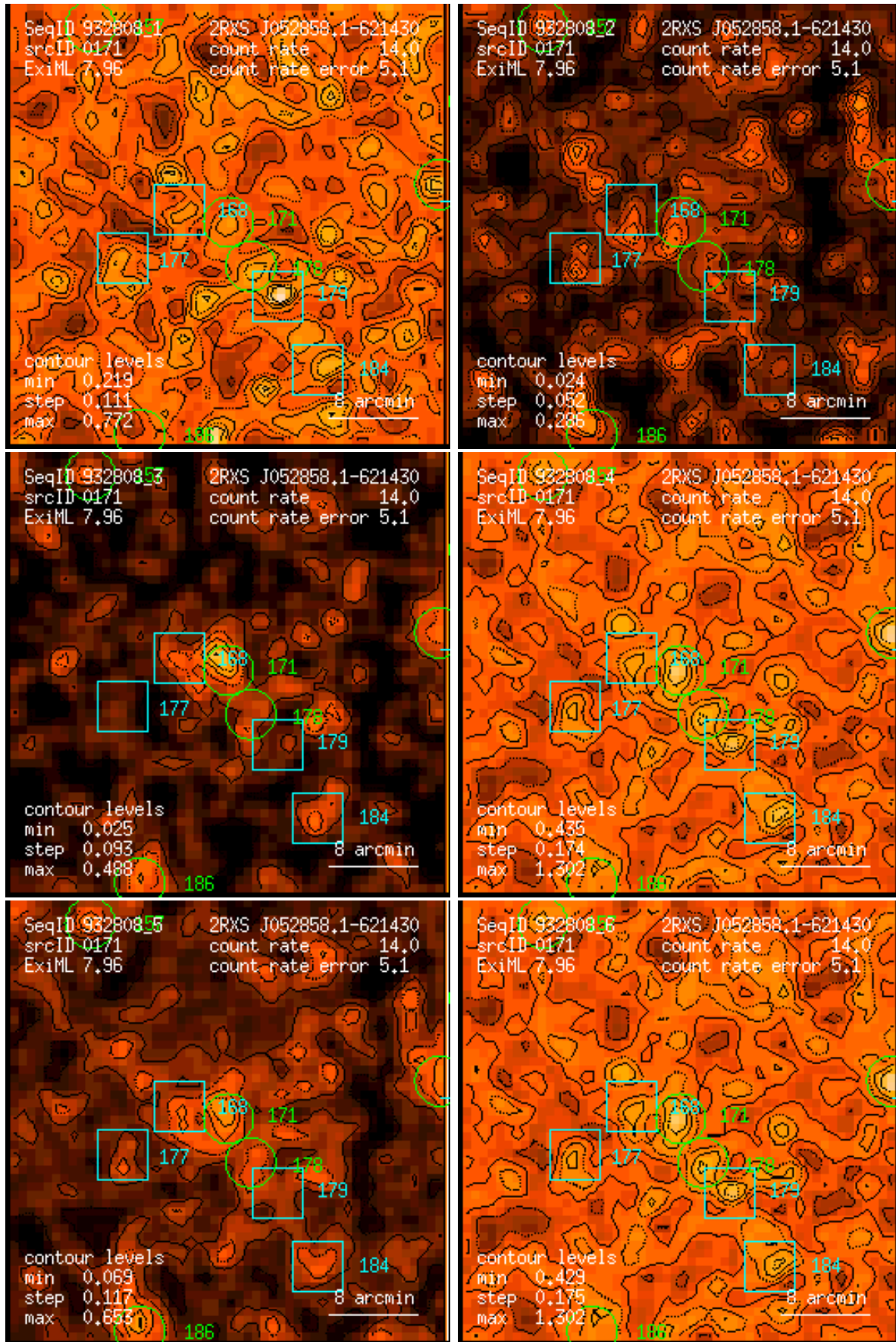
Figure 171: RASS 932808: detection 0171: band rate images, Gaussian filter: (1) PSPC channels 11 – 41, (2) 52 – 90, (3) 91 – 201, (4) 11 – 235, (5) 52 – 201, (6) 11 – 201. Broad band rates in counts/ks. Band rate contour levels in counts/ks/arcmin 2 .
