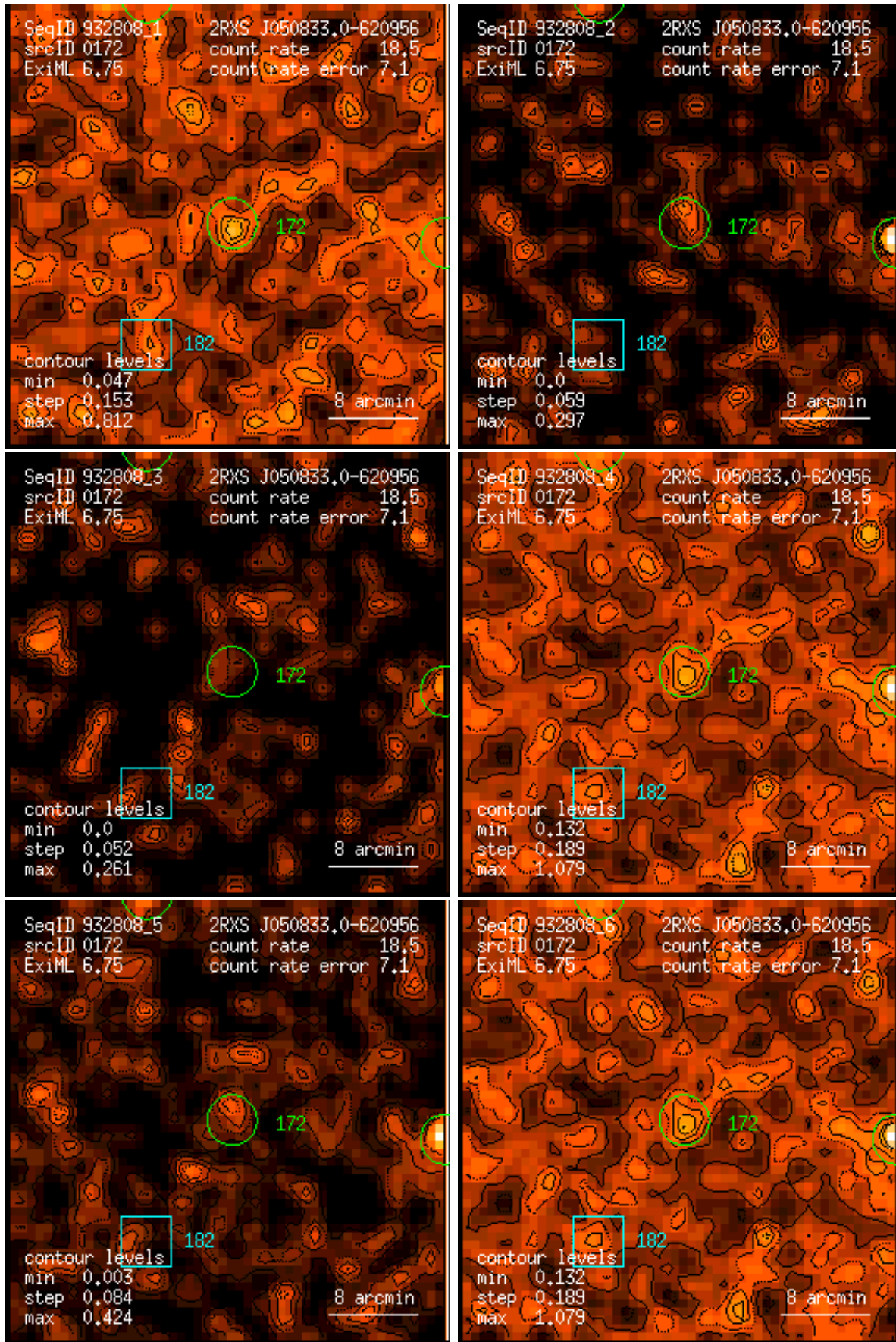
Figure 172: RASS 932808: detection 0172: band rate images, Gaussian filter: (1) PSPC channels 11 – 41, (2) 52 – 90, (3) 91 – 201, (4) 11 – 235, (5) 52 – 201, (6) 11 – 201. Broad band rates in counts/ks. Band rate contour levels in counts/ks/arcmin 2 .
