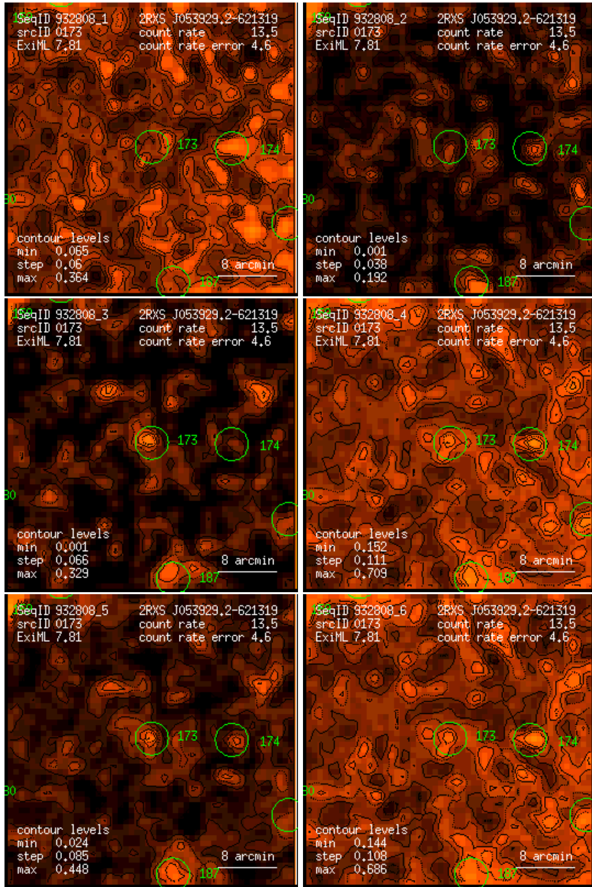
Figure 173: RASS 932808: detection 0173: band rate images, Gaussian filter: (1) PSPC channels 11 – 41, (2) 52 – 90, (3) 91 – 201, (4) 11 – 235, (5) 52 – 201, (6) 11 – 201. Broad band rates in counts/ks. Band rate contour levels in counts/ks/arcmin 2 .
