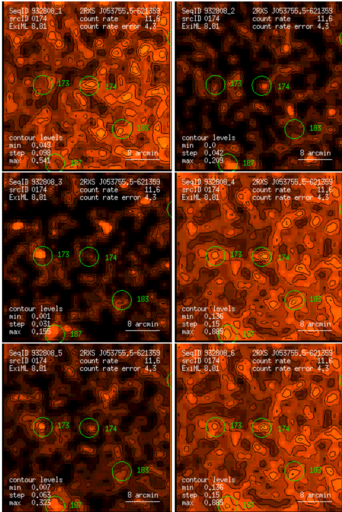
Figure 174: RASS 932808: detection 0174: band rate images, Gaussian filter: (1) PSPC channels 11 – 41, (2) 52 – 90, (3) 91 – 201, (4) 11 – 235, (5) 52 – 201, (6) 11 – 201. Broad band rates in counts/ks. Band rate contour levels in counts/ks/arcmin 2 .
