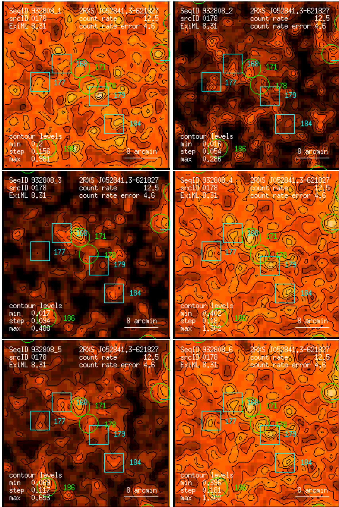
Figure 178: RASS 932808: detection 0178: band rate images, Gaussian filter: (1) PSPC channels 11 – 41, (2) 52 – 90, (3) 91 – 201, (4) 11 – 235, (5) 52 – 201, (6) 11 – 201. Broad band rates in counts/ks. Band rate contour levels in counts/ks/arcmin 2 .
