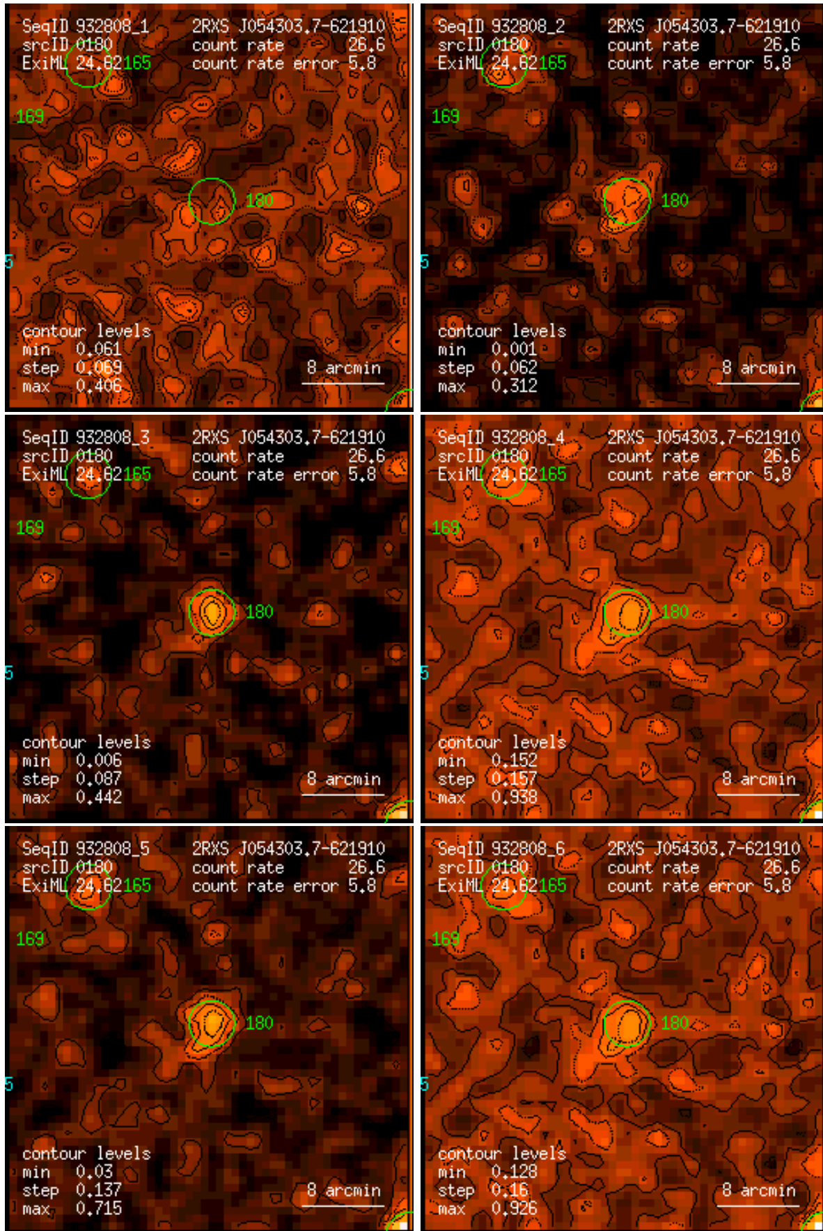
Figure 180: RASS 932808: detection 0180: band rate images, Gaussian filter: (1) PSPC channels 11 – 41, (2) 52 – 90, (3) 91 – 201, (4) 11 – 235, (5) 52 – 201, (6) 11 – 201. Broad band rates in counts/ks. Band rate contour levels in counts/ks/arcmin 2 .
