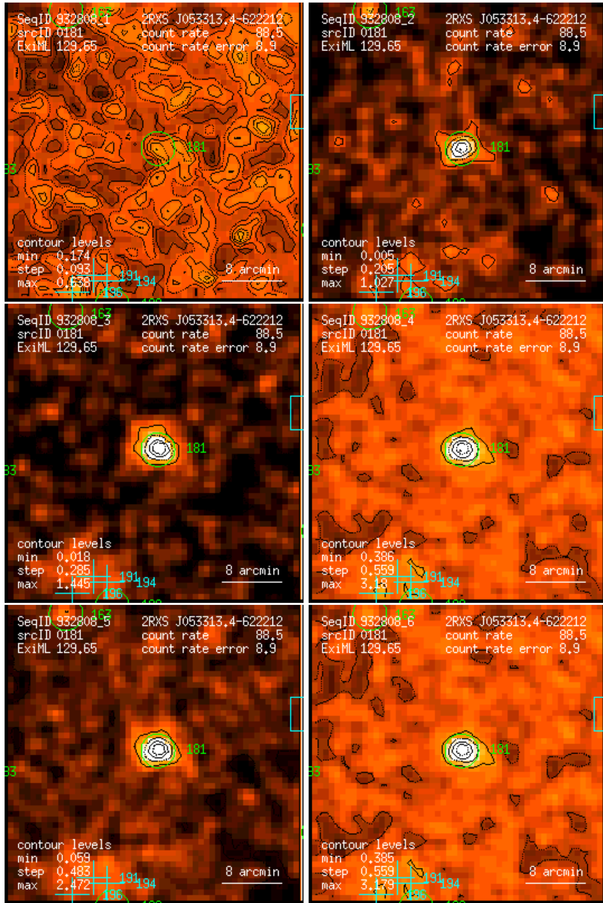
Figure 181: RASS 932808: detection 0181: band rate images, Gaussian filter: (1) PSPC channels 11 – 41, (2) 52 – 90, (3) 91 – 201, (4) 11 – 235, (5) 52 – 201, (6) 11 – 201. Broad band rates in counts/ks. Band rate contour levels in counts/ks/arcmin 2 .
