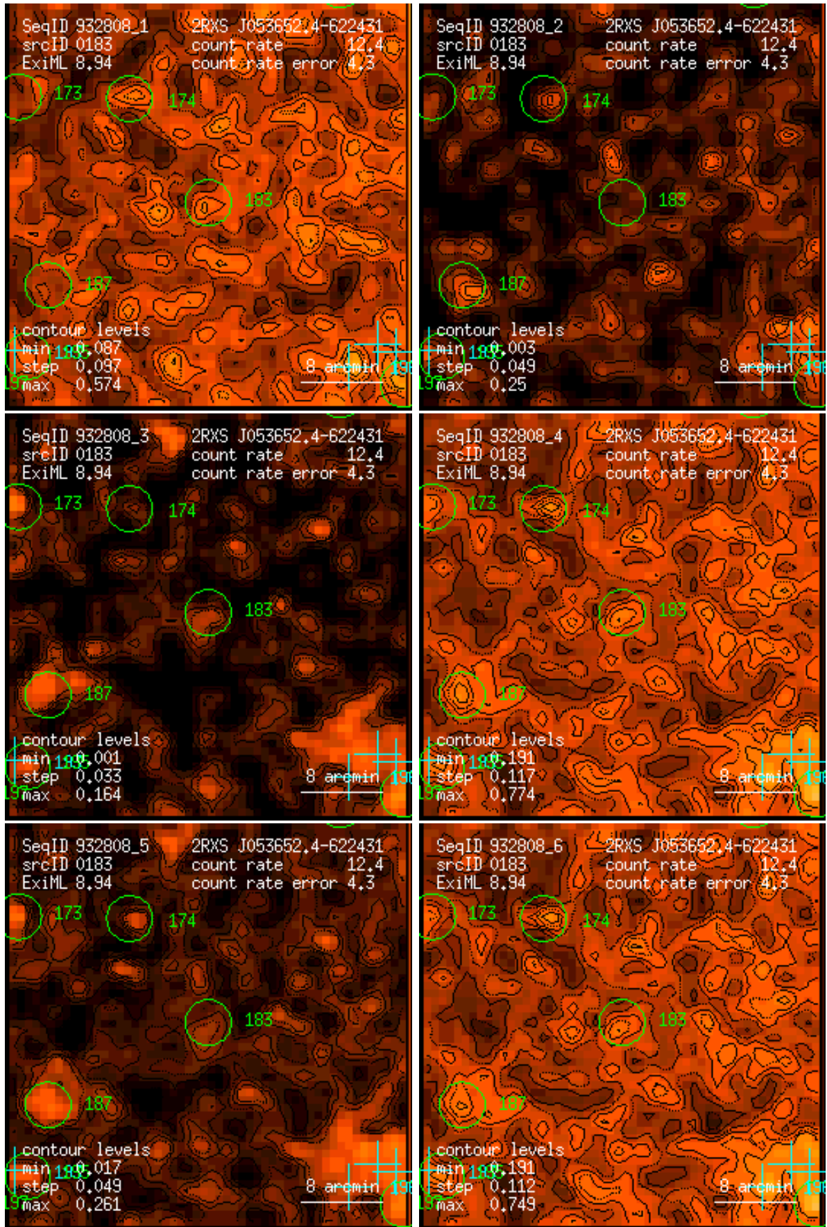
Figure 183: RASS 932808: detection 0183: band rate images, Gaussian filter: (1) PSPC channels 11 – 41, (2) 52 – 90, (3) 91 – 201, (4) 11 – 235, (5) 52 – 201, (6) 11 – 201. Broad band rates in counts/ks. Band rate contour levels in counts/ks/arcmin 2 .
