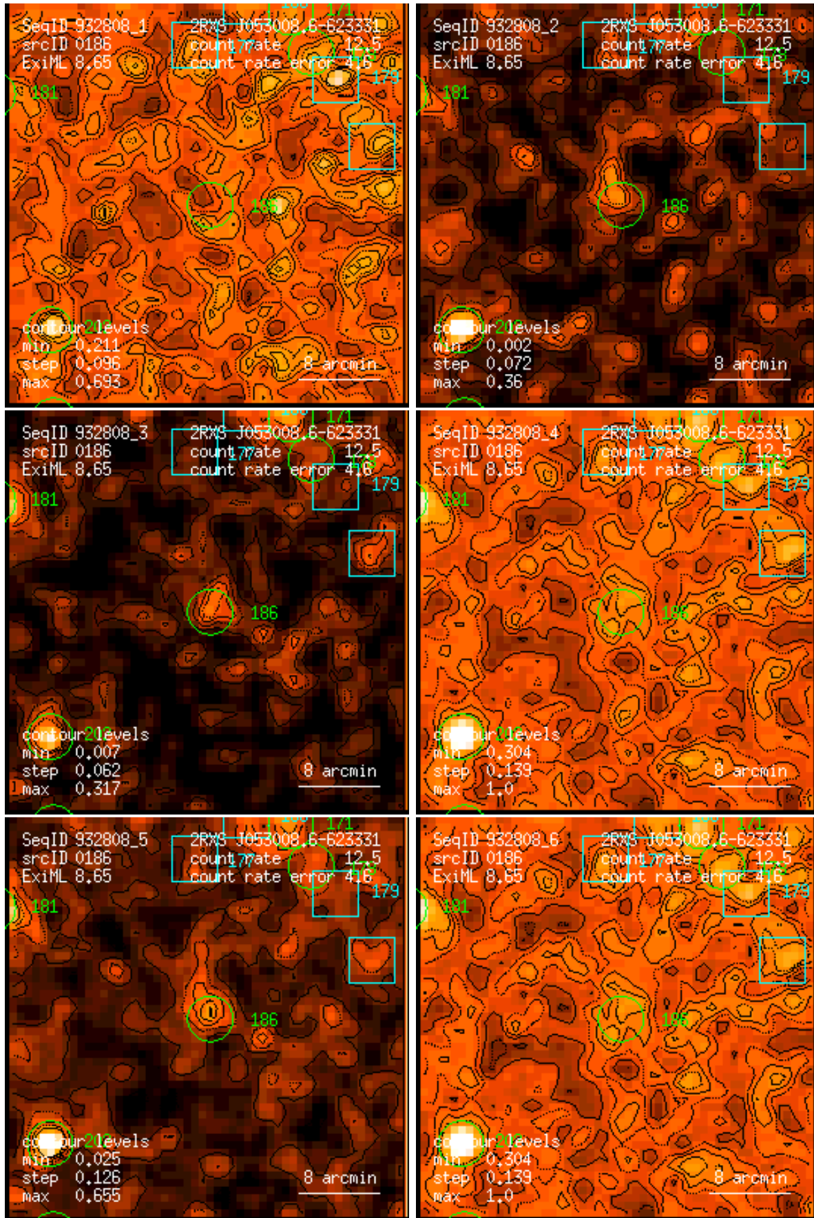
Figure 186: RASS 932808: detection 0186: band rate images, Gaussian filter: (1) PSPC channels 11 – 41, (2) 52 – 90, (3) 91 – 201, (4) 11 – 235, (5) 52 – 201, (6) 11 – 201. Broad band rates in counts/ks. Band rate contour levels in counts/ks/arcmin 2 .
