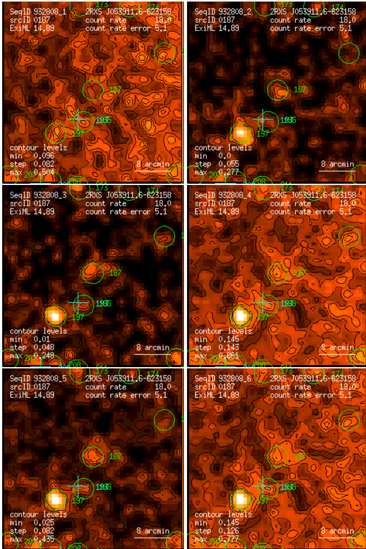
Figure 187: RASS 932808: detection 0187: band rate images, Gaussian filter: (1) PSPC channels 11 – 41, (2) 52 – 90, (3) 91 – 201, (4) 11 – 235, (5) 52 – 201, (6) 11 – 201. Broad band rates in counts/ks. Band rate contour levels in counts/ks/arcmin 2 .
