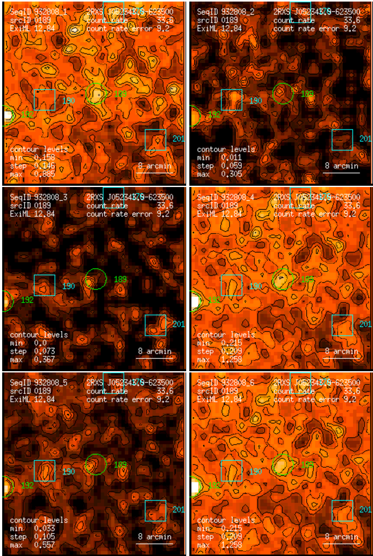
Figure 189: RASS 932808: detection 0189: band rate images, Gaussian filter: (1) PSPC channels 11 – 41, (2) 52 – 90, (3) 91 – 201, (4) 11 – 235, (5) 52 – 201, (6) 11 – 201. Broad band rates in counts/ks. Band rate contour levels in counts/ks/arcmin 2 .
