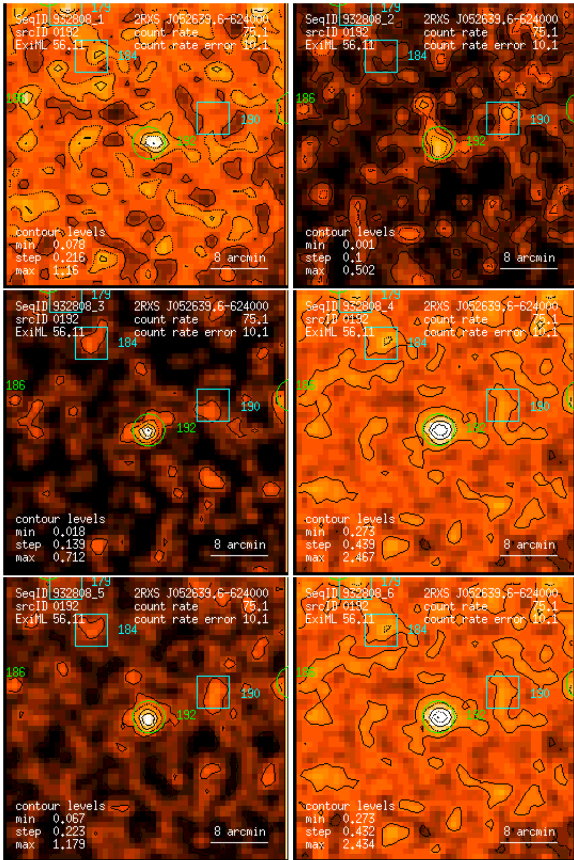
Figure 192: RASS 932808: detection 0192: band rate images, Gaussian filter: (1) PSPC channels 11 – 41, (2) 52 – 90, (3) 91 – 201, (4) 11 – 235, (5) 52 – 201, (6) 11 – 201. Broad band rates in counts/ks. Band rate contour levels in counts/ks/arcmin 2 .
