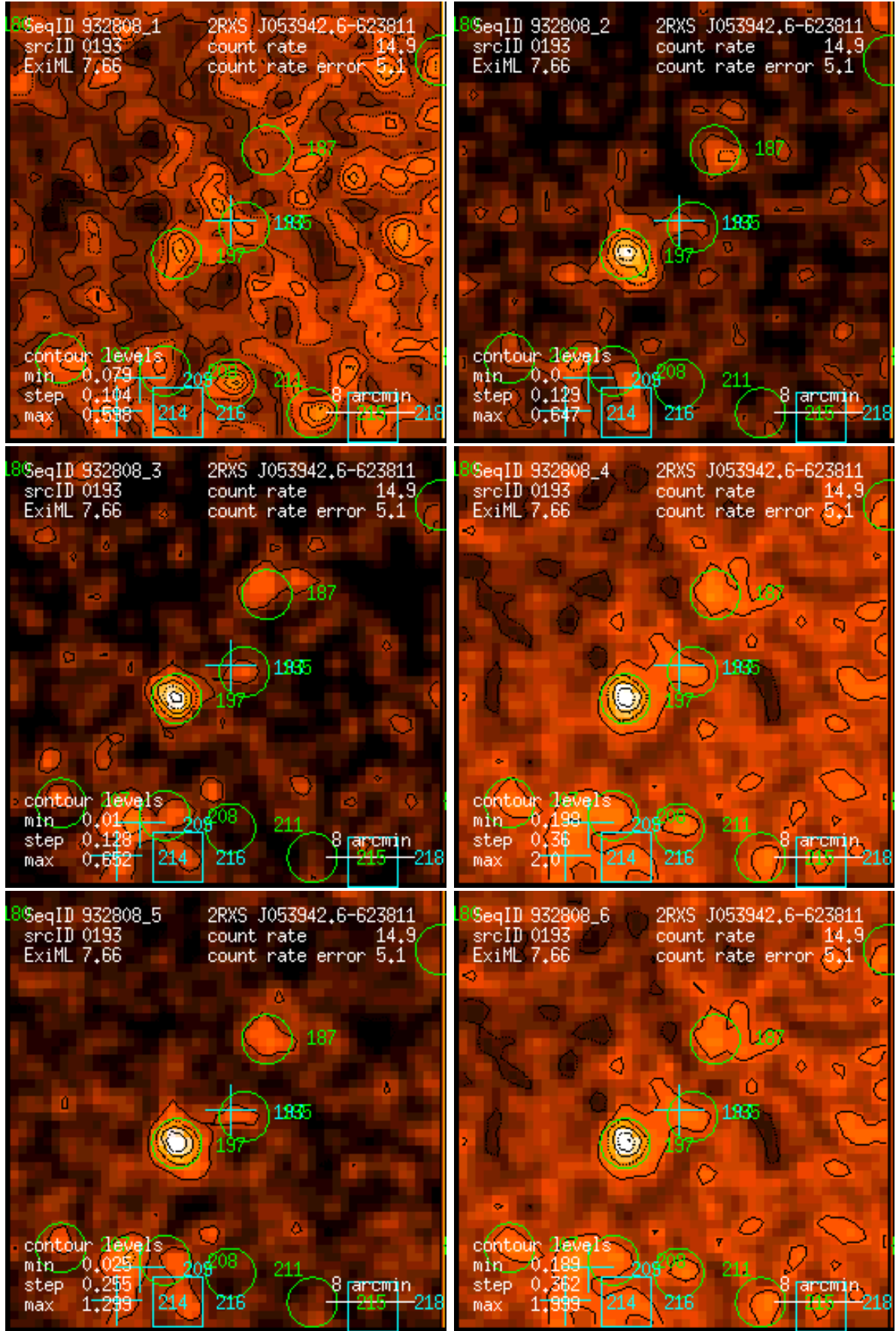
Figure 193: RASS 932808: detection 0193: band rate images, Gaussian filter: (1) PSPC channels 11 – 41, (2) 52 – 90, (3) 91 – 201, (4) 11 – 235, (5) 52 – 201, (6) 11 – 201. Broad band rates in counts/ks. Band rate contour levels in counts/ks/arcmin 2 .
