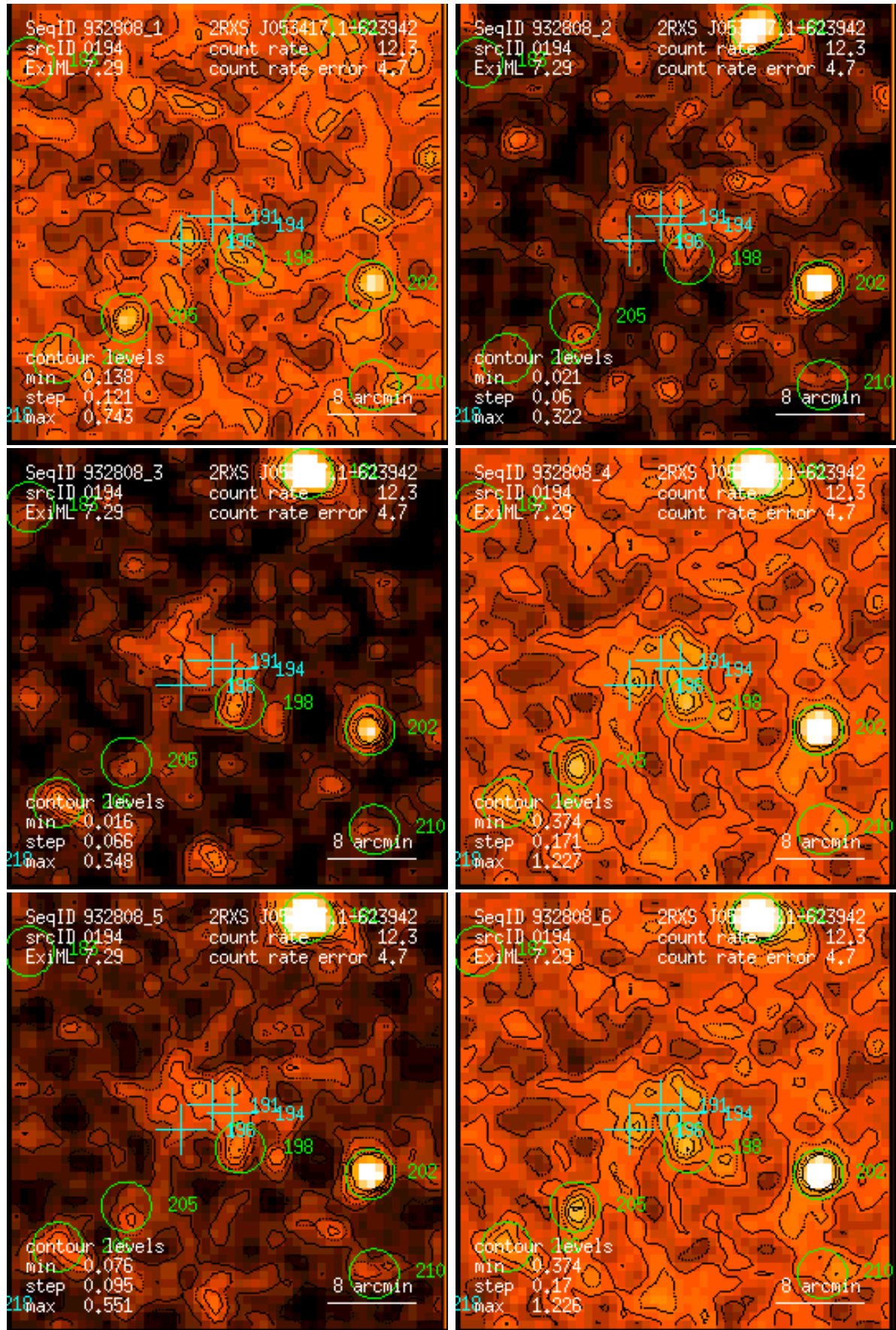
Figure 194: RASS 932808: detection 0194: band rate images, Gaussian filter: (1) PSPC channels 11 – 41, (2) 52 – 90, (3) 91 – 201, (4) 11 – 235, (5) 52 – 201, (6) 11 – 201. Broad band rates in counts/ks. Band rate contour levels in counts/ks/arcmin 2 .
