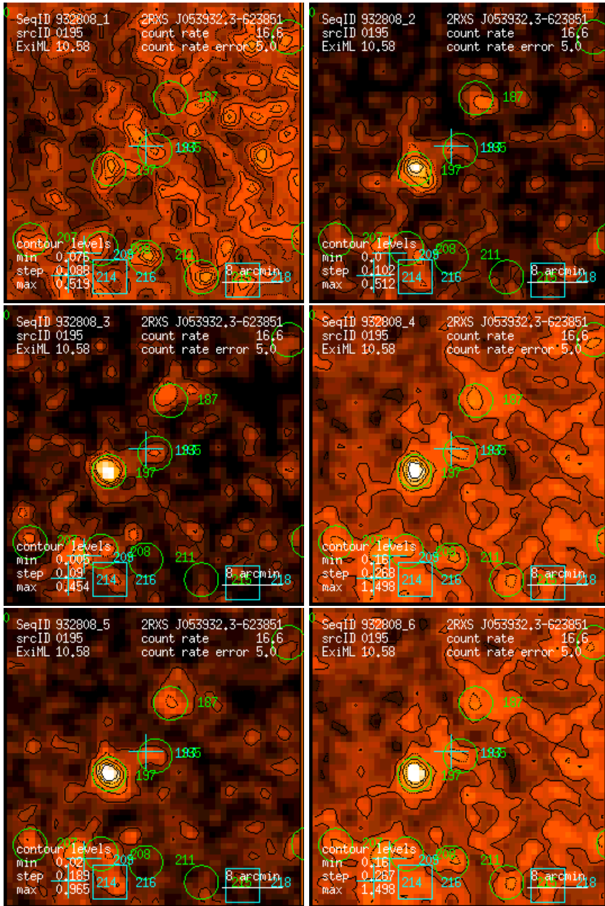
Figure 195: RASS 932808: detection 0195: band rate images, Gaussian filter: (1) PSPC channels 11 – 41, (2) 52 – 90, (3) 91 – 201, (4) 11 – 235, (5) 52 – 201, (6) 11 – 201. Broad band rates in counts/ks. Band rate contour levels in counts/ks/arcmin 2 .
