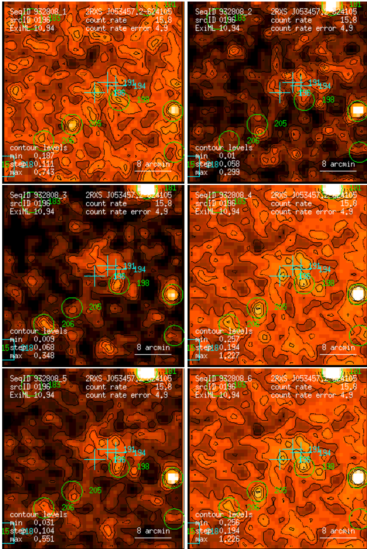
Figure 196: RASS 932808: detection 0196: band rate images, Gaussian filter: (1) PSPC channels 11 – 41, (2) 52 – 90, (3) 91 – 201, (4) 11 – 235, (5) 52 – 201, (6) 11 – 201. Broad band rates in counts/ks. Band rate contour levels in counts/ks/arcmin 2 .
