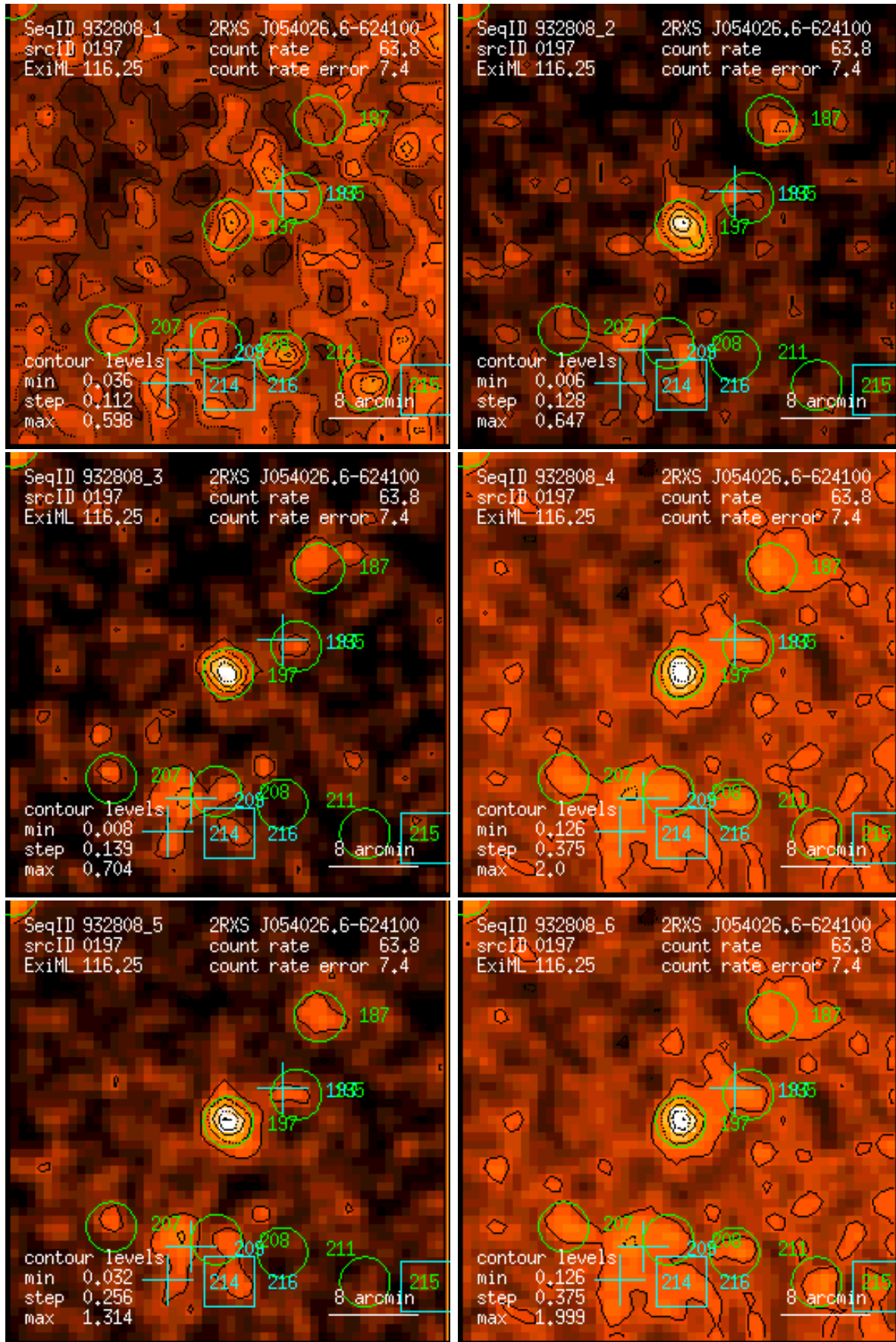
Figure 197: RASS 932808: detection 0197: band rate images, Gaussian filter: (1) PSPC channels 11 – 41, (2) 52 – 90, (3) 91 – 201, (4) 11 – 235, (5) 52 – 201, (6) 11 – 201. Broad band rates in counts/ks. Band rate contour levels in counts/ks/arcmin 2 .
