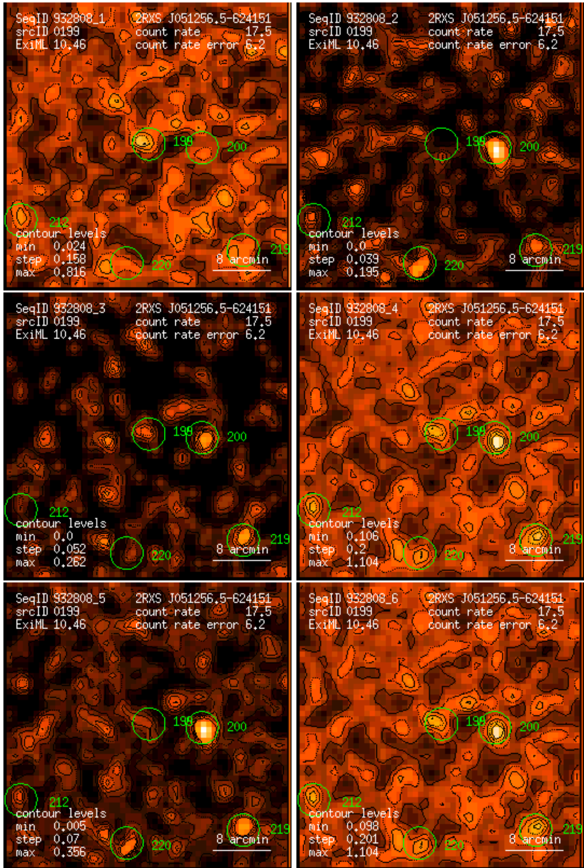
Figure 199: RASS 932808: detection 0199: band rate images, Gaussian filter: (1) PSPC channels 11 – 41, (2) 52 – 90, (3) 91 – 201, (4) 11 – 235, (5) 52 – 201, (6) 11 – 201. Broad band rates in counts/ks. Band rate contour levels in counts/ks/arcmin 2 .
