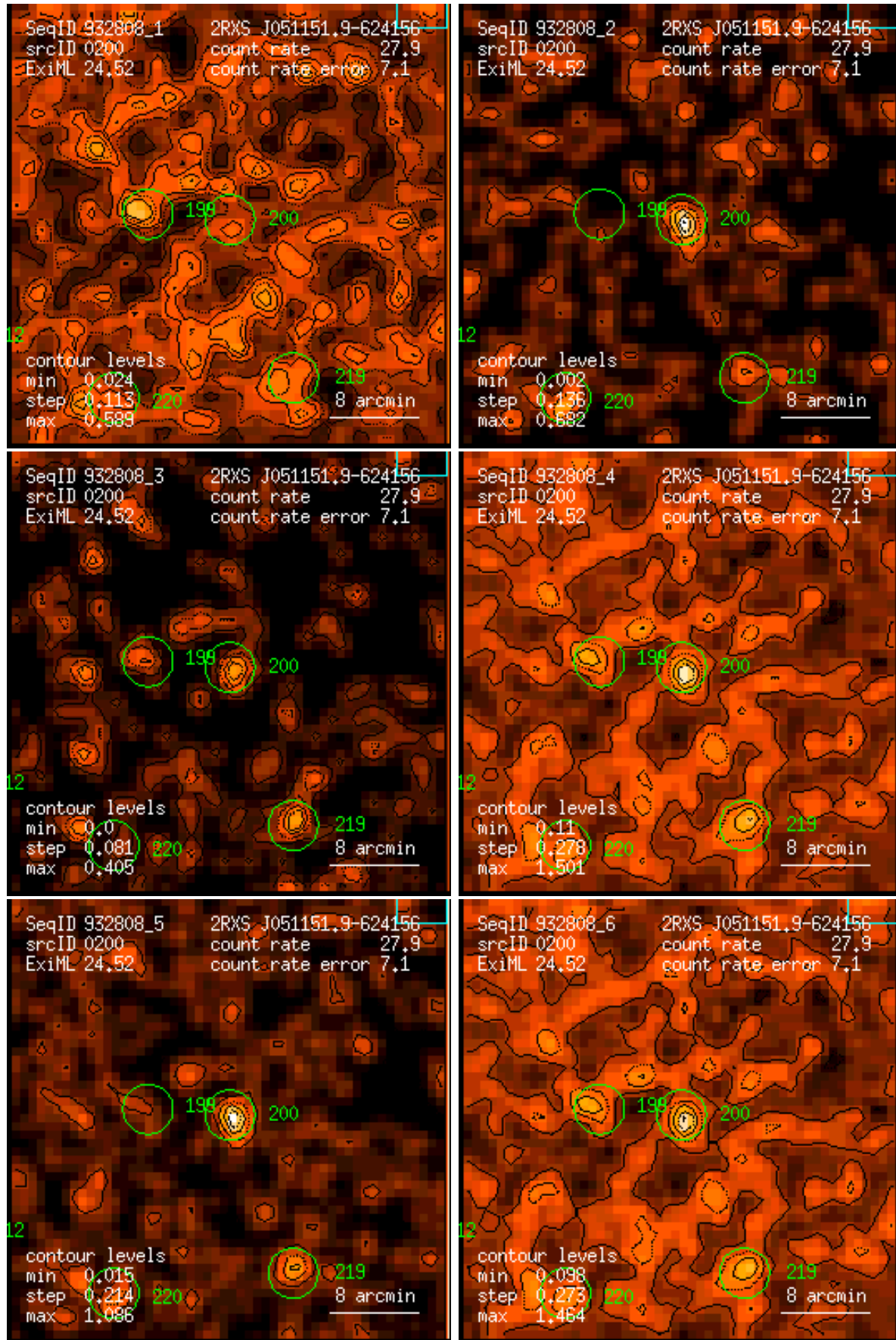
Figure 200: RASS 932808: detection 0200: band rate images, Gaussian filter: (1) PSPC channels 11 – 41, (2) 52 – 90, (3) 91 – 201, (4) 11 – 235, (5) 52 – 201, (6) 11 – 201. Broad band rates in counts/ks. Band rate contour levels in counts/ks/arcmin 2 .
