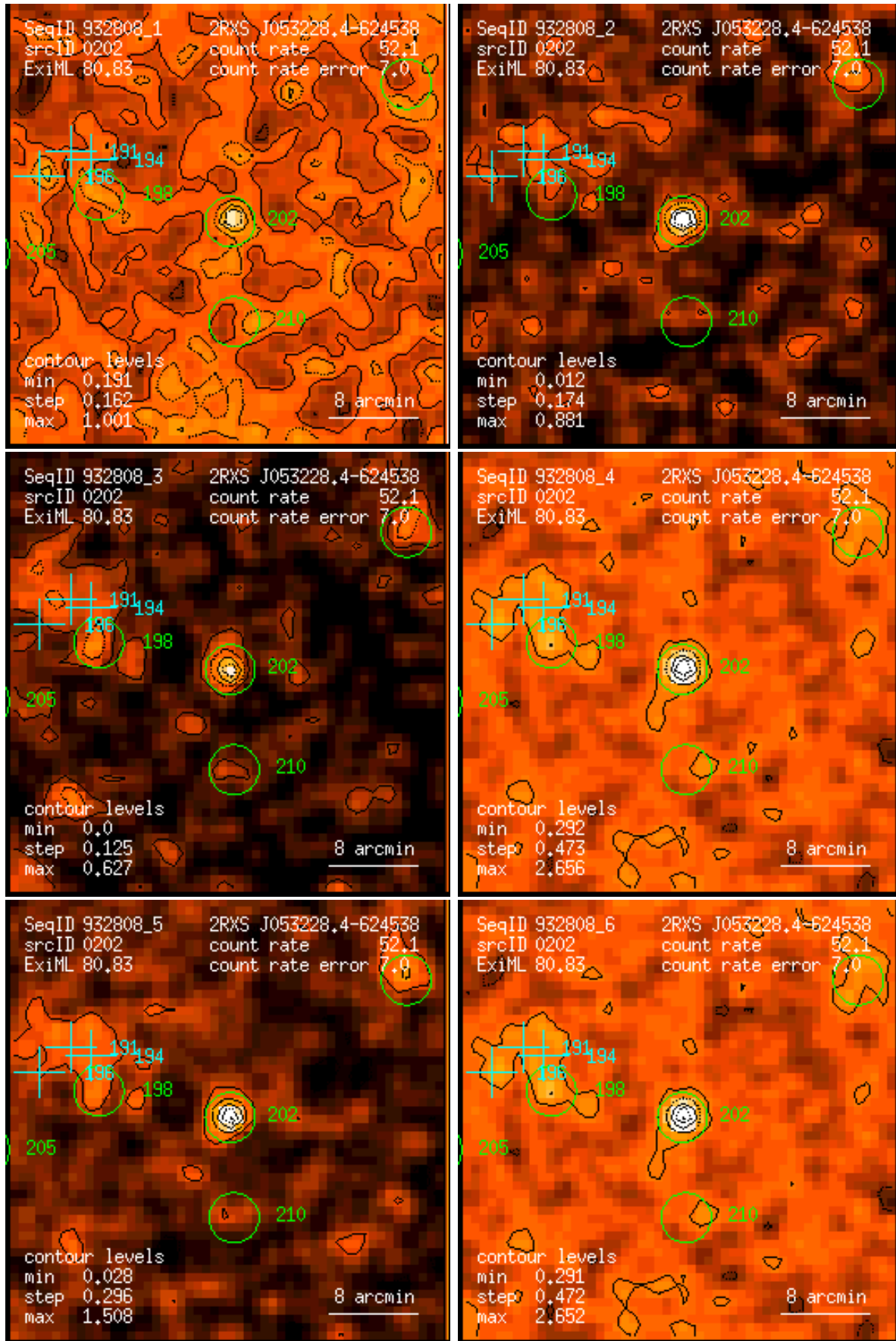
Figure 202: RASS 932808: detection 0202: band rate images, Gaussian filter: (1) PSPC channels 11 – 41, (2) 52 – 90, (3) 91 – 201, (4) 11 – 235, (5) 52 – 201, (6) 11 – 201. Broad band rates in counts/ks. Band rate contour levels in counts/ks/arcmin 2 .
