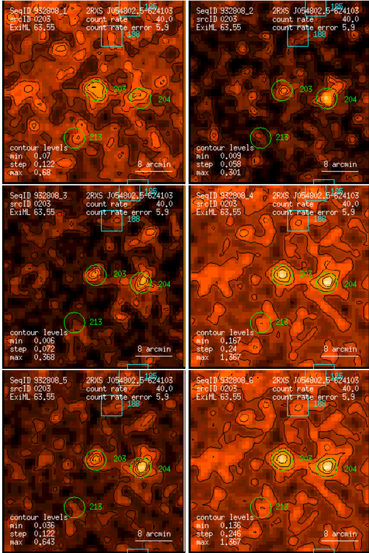
Figure 203: RASS 932808: detection 0203: band rate images, Gaussian filter: (1) PSPC channels 11 – 41, (2) 52 – 90, (3) 91 – 201, (4) 11 – 235, (5) 52 – 201, (6) 11 – 201. Broad band rates in counts/ks. Band rate contour levels in counts/ks/arcmin 2 .
