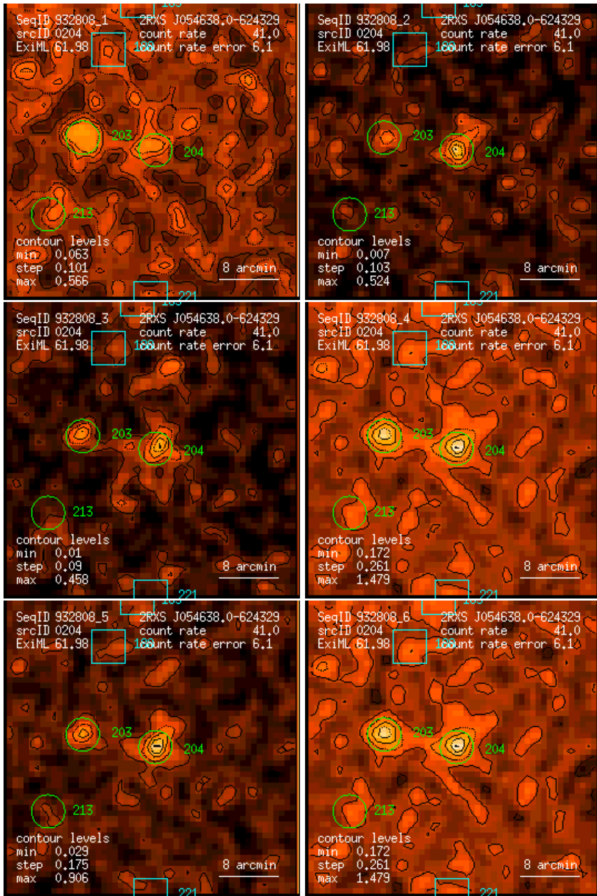
Figure 204: RASS 932808: detection 0204: band rate images, Gaussian filter: (1) PSPC channels 11 – 41, (2) 52 – 90, (3) 91 – 201, (4) 11 – 235, (5) 52 – 201, (6) 11 – 201. Broad band rates in counts/ks. Band rate contour levels in counts/ks/arcmin 2 .
