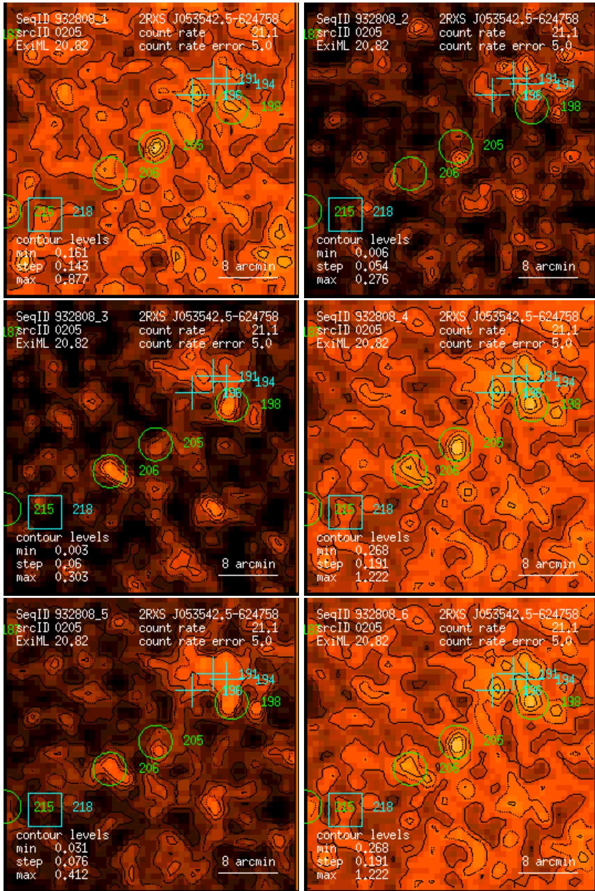
Figure 205: RASS 932808: detection 0205: band rate images, Gaussian filter: (1) PSPC channels 11 – 41, (2) 52 – 90, (3) 91 – 201, (4) 11 – 235, (5) 52 – 201, (6) 11 – 201. Broad band rates in counts/ks. Band rate contour levels in counts/ks/arcmin 2 .
