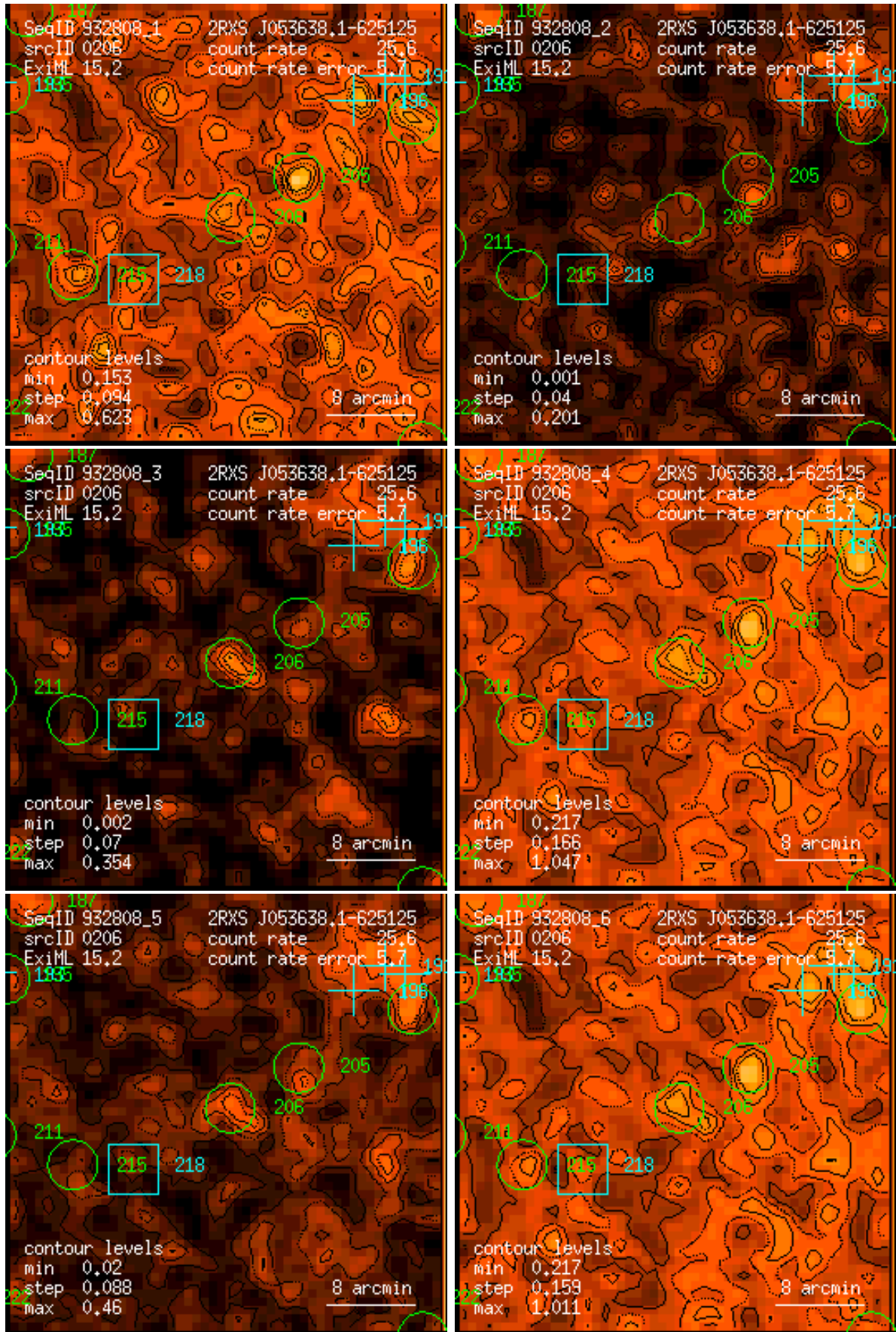
Figure 206: RASS 932808: detection 0206: band rate images, Gaussian filter: (1) PSPC channels 11 – 41, (2) 52 – 90, (3) 91 – 201, (4) 11 – 235, (5) 52 – 201, (6) 11 – 201. Broad band rates in counts/ks. Band rate contour levels in counts/ks/arcmin 2 .
