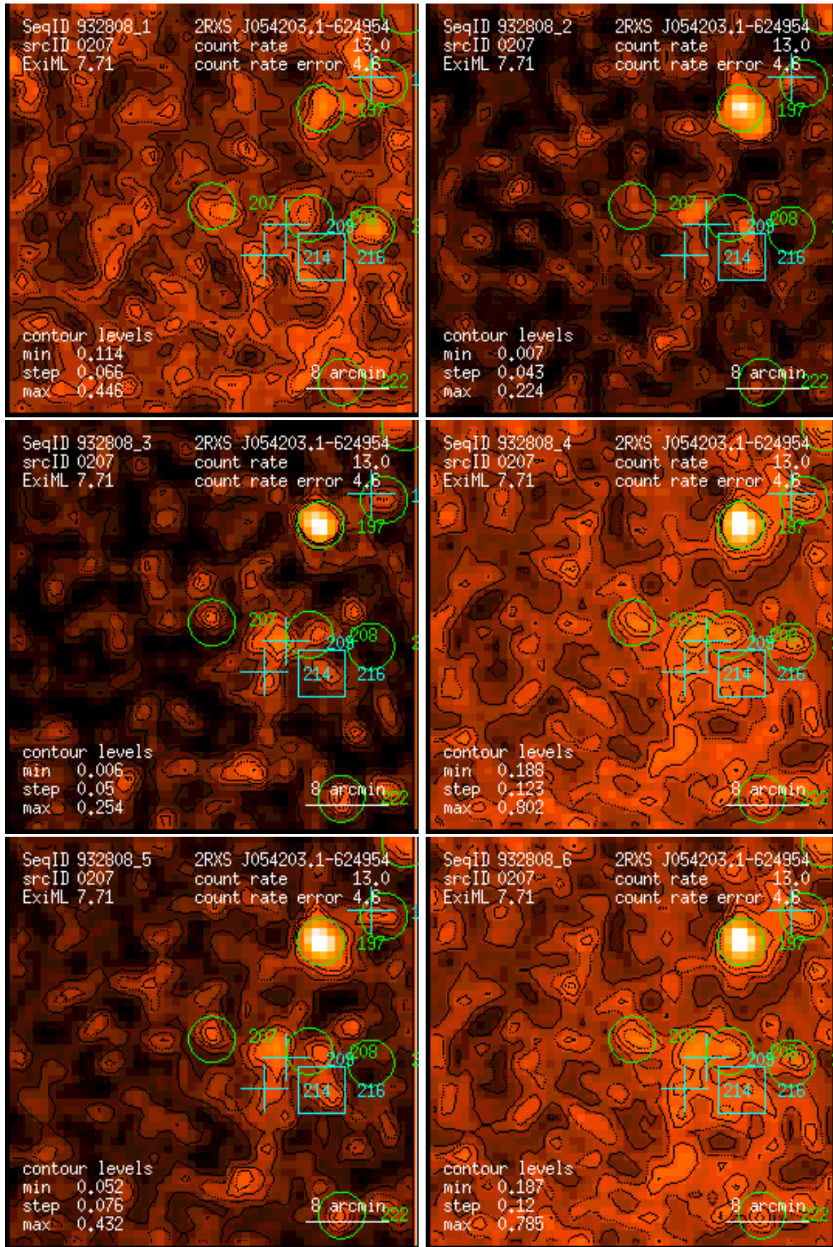
Figure 207: RASS 932808: detection 0207: band rate images, Gaussian filter: (1) PSPC channels 11 – 41, (2) 52 – 90, (3) 91 – 201, (4) 11 – 235, (5) 52 – 201, (6) 11 – 201. Broad band rates in counts/ks. Band rate contour levels in counts/ks/arcmin 2 .
