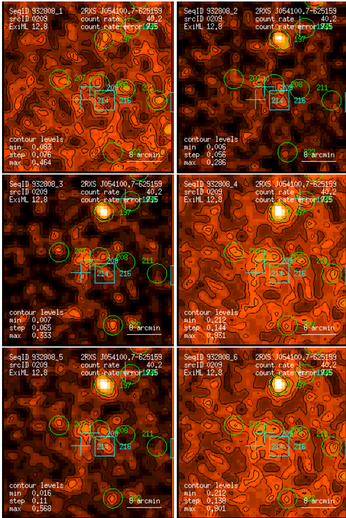
Figure 209: RASS 932808: detection 0209: band rate images, Gaussian filter: (1) PSPC channels 11 – 41, (2) 52 – 90, (3) 91 – 201, (4) 11 – 235, (5) 52 – 201, (6) 11 – 201. Broad band rates in counts/ks. Band rate contour levels in counts/ks/arcmin 2 .
