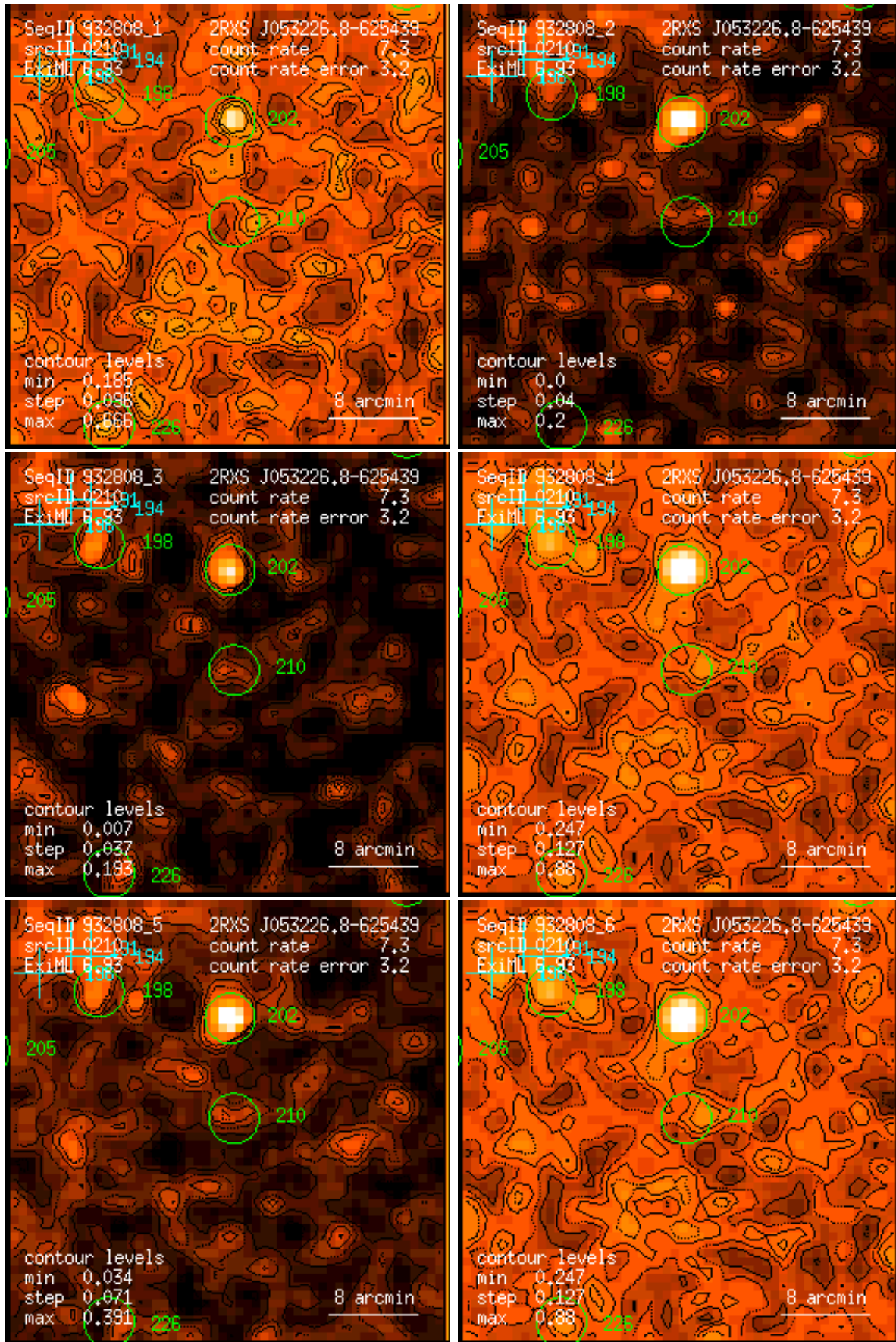
Figure 210: RASS 932808: detection 0210: band rate images, Gaussian filter: (1) PSPC channels 11 – 41, (2) 52 – 90, (3) 91 – 201, (4) 11 – 235, (5) 52 – 201, (6) 11 – 201. Broad band rates in counts/ks. Band rate contour levels in counts/ks/arcmin 2 .
