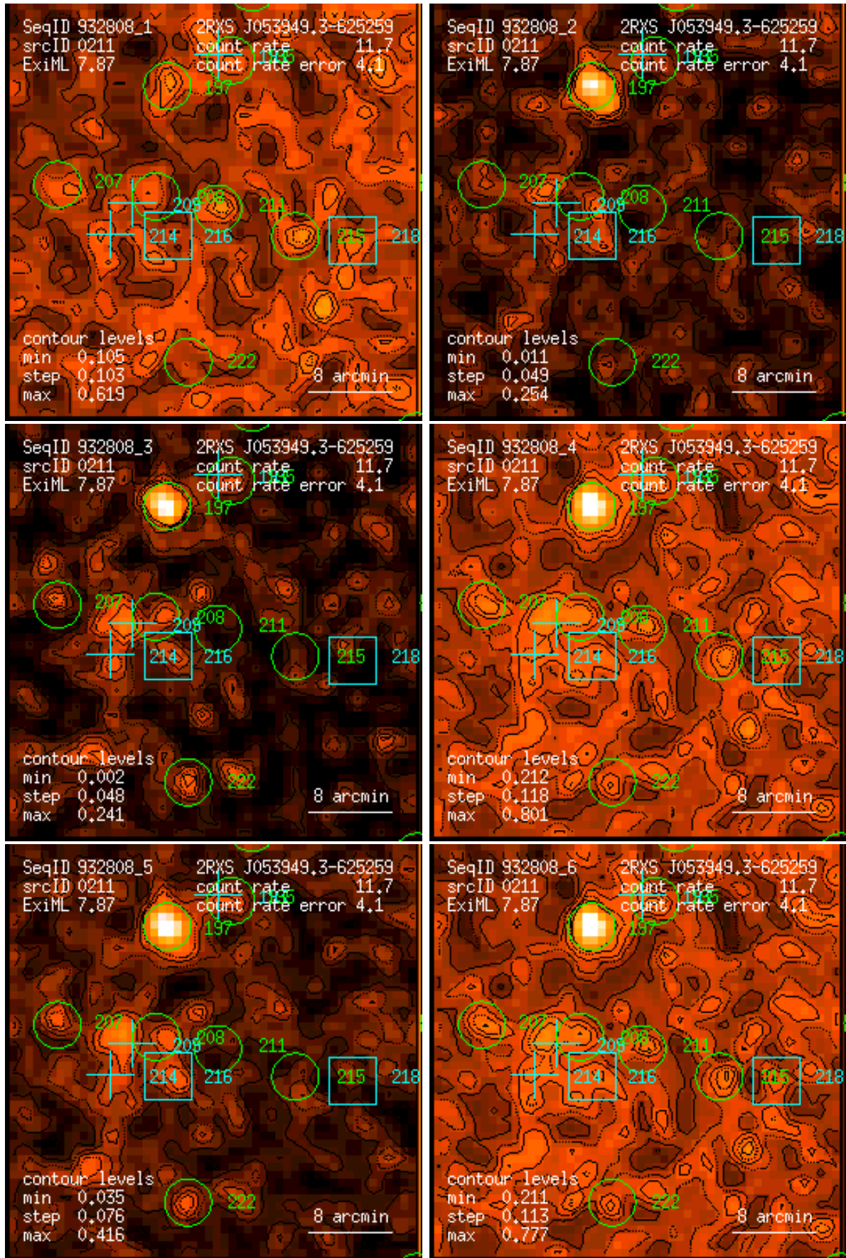
Figure 211: RASS 932808: detection 0211: band rate images, Gaussian filter: (1) PSPC channels 11 – 41, (2) 52 – 90, (3) 91 – 201, (4) 11 – 235, (5) 52 – 201, (6) 11 – 201. Broad band rates in counts/ks. Band rate contour levels in counts/ks/arcmin 2 .
