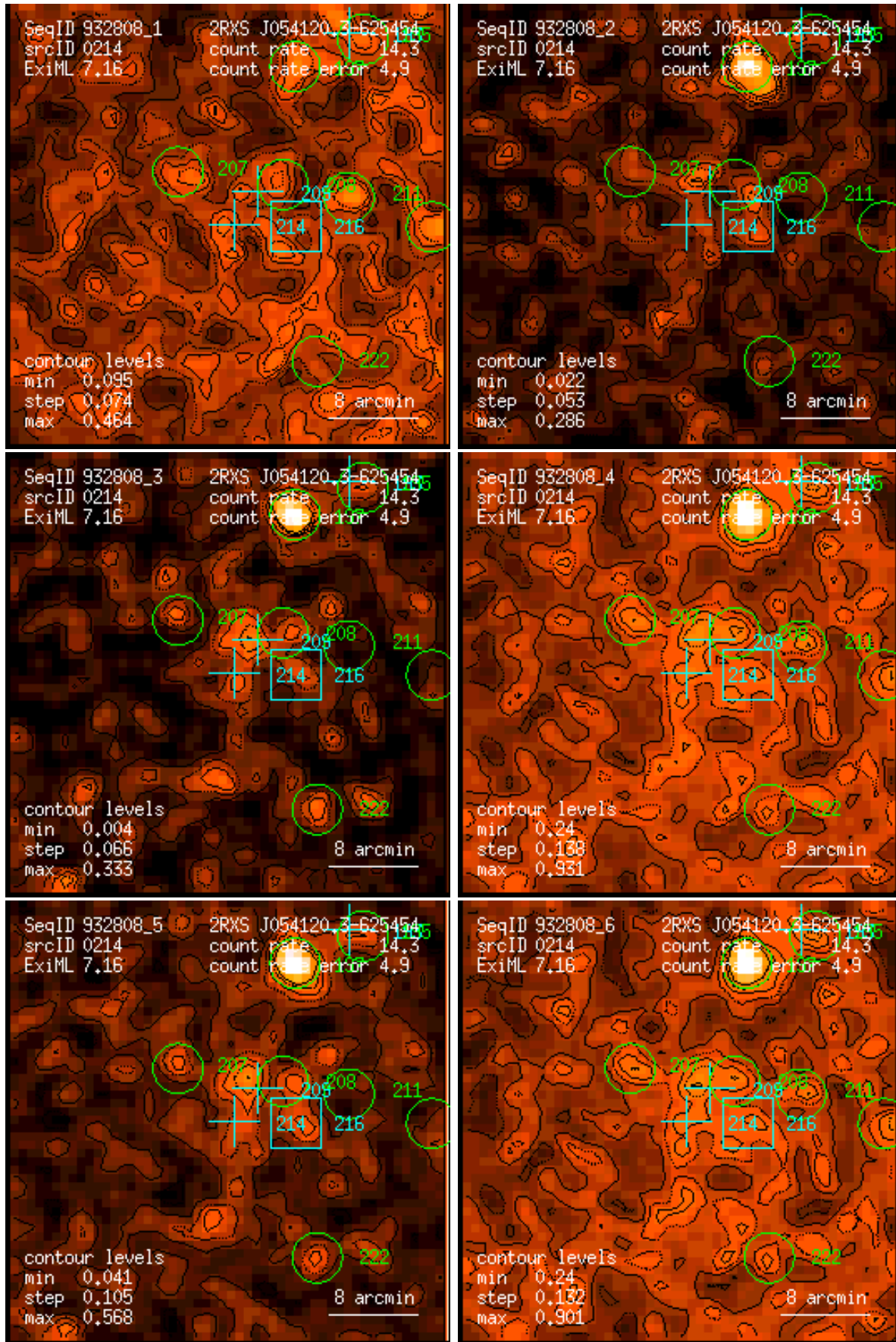
Figure 214: RASS 932808: detection 0214: band rate images, Gaussian filter: (1) PSPC channels 11 – 41, (2) 52 – 90, (3) 91 – 201, (4) 11 – 235, (5) 52 – 201, (6) 11 – 201. Broad band rates in counts/ks. Band rate contour levels in counts/ks/arcmin 2 .
