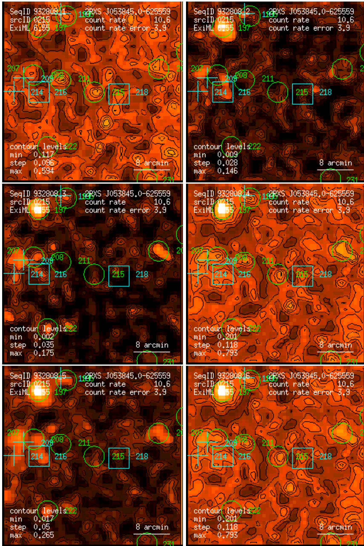
Figure 215: RASS 932808: detection 0215: band rate images, Gaussian filter: (1) PSPC channels 11 – 41, (2) 52 – 90, (3) 91 – 201, (4) 11 – 235, (5) 52 – 201, (6) 11 – 201. Broad band rates in counts/ks. Band rate contour levels in counts/ks/arcmin 2 .
