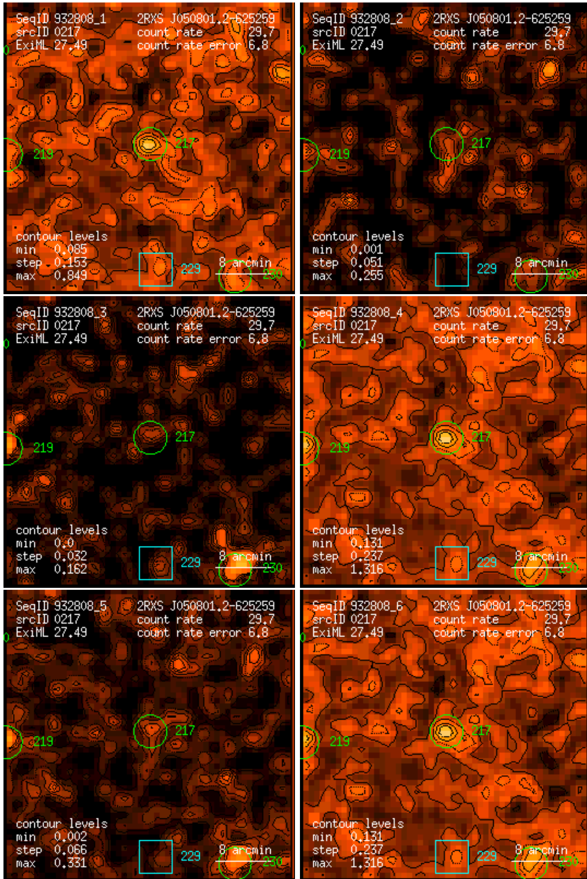
Figure 217: RASS 932808: detection 0217: band rate images, Gaussian filter: (1) PSPC channels 11 – 41, (2) 52 – 90, (3) 91 – 201, (4) 11 – 235, (5) 52 – 201, (6) 11 – 201. Broad band rates in counts/ks. Band rate contour levels in counts/ks/arcmin 2 .
