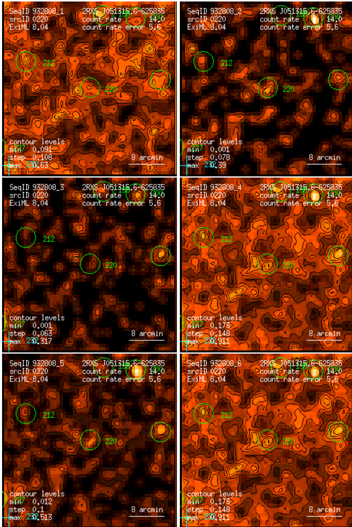
Figure 220: RASS 932808: detection 0220: band rate images, Gaussian filter: (1) PSPC channels 11 – 41, (2) 52 – 90, (3) 91 – 201, (4) 11 – 235, (5) 52 – 201, (6) 11 – 201. Broad band rates in counts/ks. Band rate contour levels in counts/ks/arcmin 2 .
