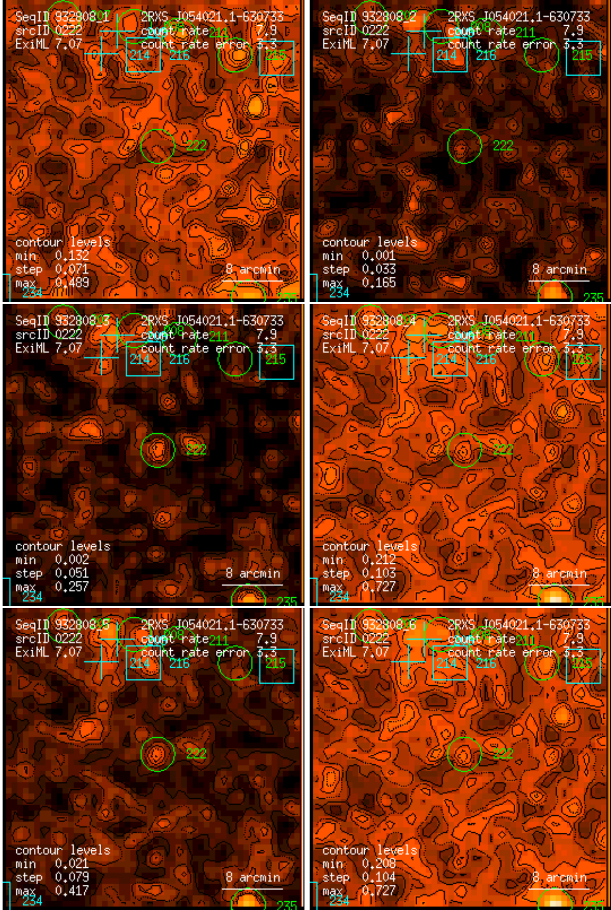
Figure 222: RASS 932808: detection 0222: band rate images, Gaussian filter: (1) PSPC channels 11 – 41, (2) 52 – 90, (3) 91 – 201, (4) 11 – 235, (5) 52 – 201, (6) 11 – 201. Broad band rates in counts/ks. Band rate contour levels in counts/ks/arcmin 2 .
