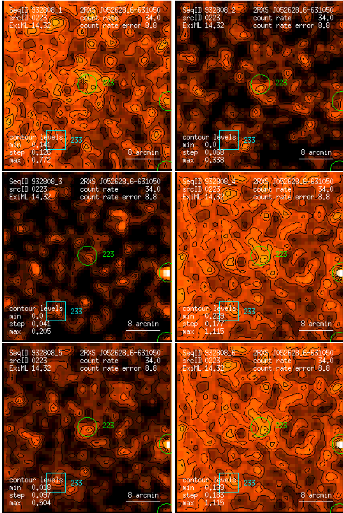
Figure 223: RASS 932808: detection 0223: band rate images, Gaussian filter: (1) PSPC channels 11 – 41, (2) 52 – 90, (3) 91 – 201, (4) 11 – 235, (5) 52 – 201, (6) 11 – 201. Broad band rates in counts/ks. Band rate contour levels in counts/ks/arcmin 2 .
