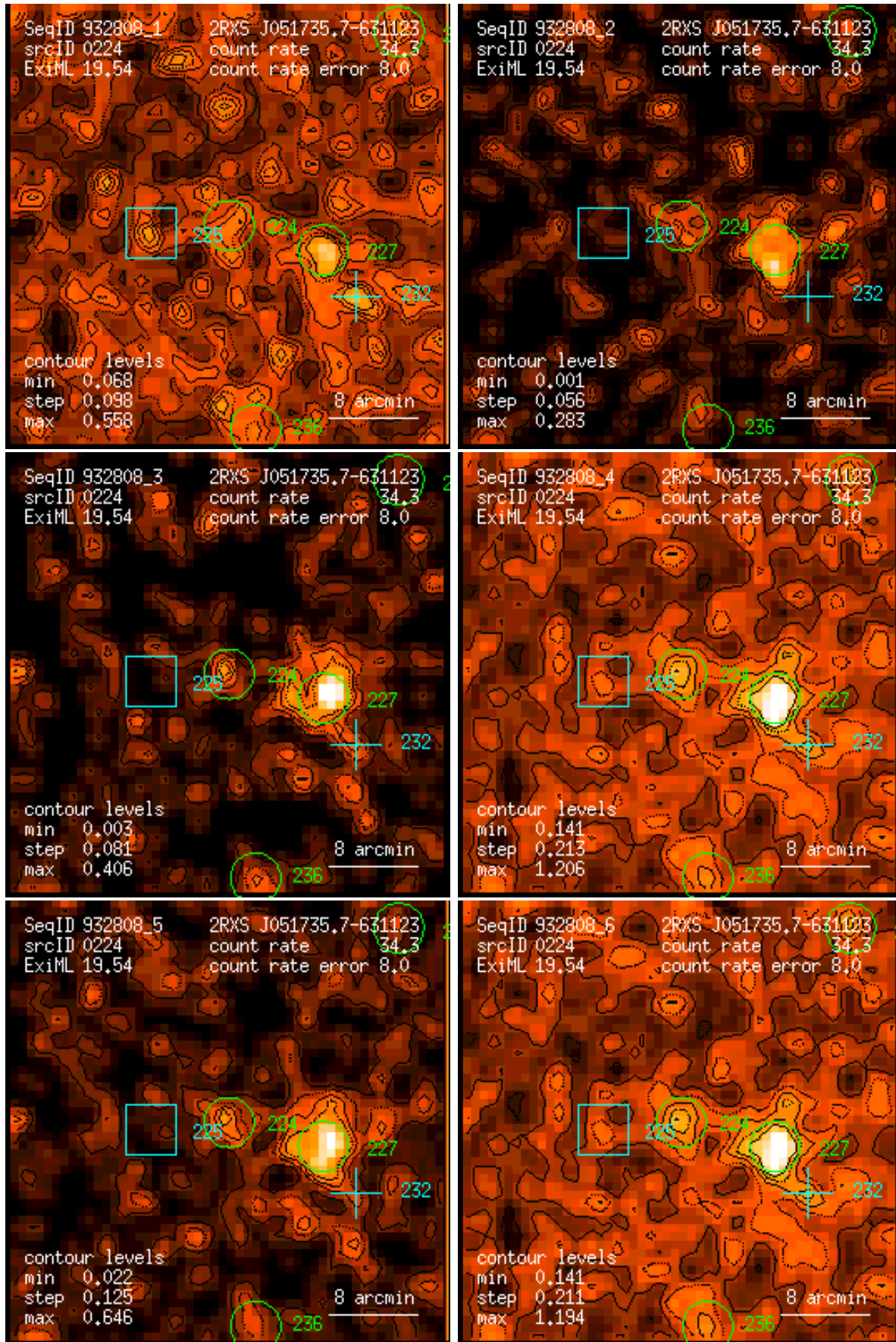
Figure 224: RASS 932808: detection 0224: band rate images, Gaussian filter: (1) PSPC channels 11 – 41, (2) 52 – 90, (3) 91 – 201, (4) 11 – 235, (5) 52 – 201, (6) 11 – 201. Broad band rates in counts/ks. Band rate contour levels in counts/ks/arcmin 2 .
