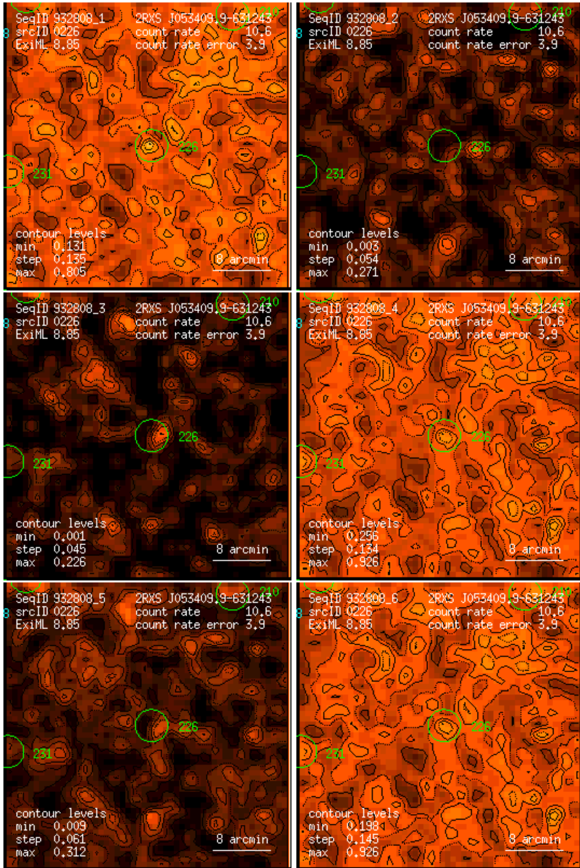
Figure 226: RASS 932808: detection 0226: band rate images, Gaussian filter: (1) PSPC channels 11 – 41, (2) 52 – 90, (3) 91 – 201, (4) 11 – 235, (5) 52 – 201, (6) 11 – 201. Broad band rates in counts/ks. Band rate contour levels in counts/ks/arcmin 2 .
