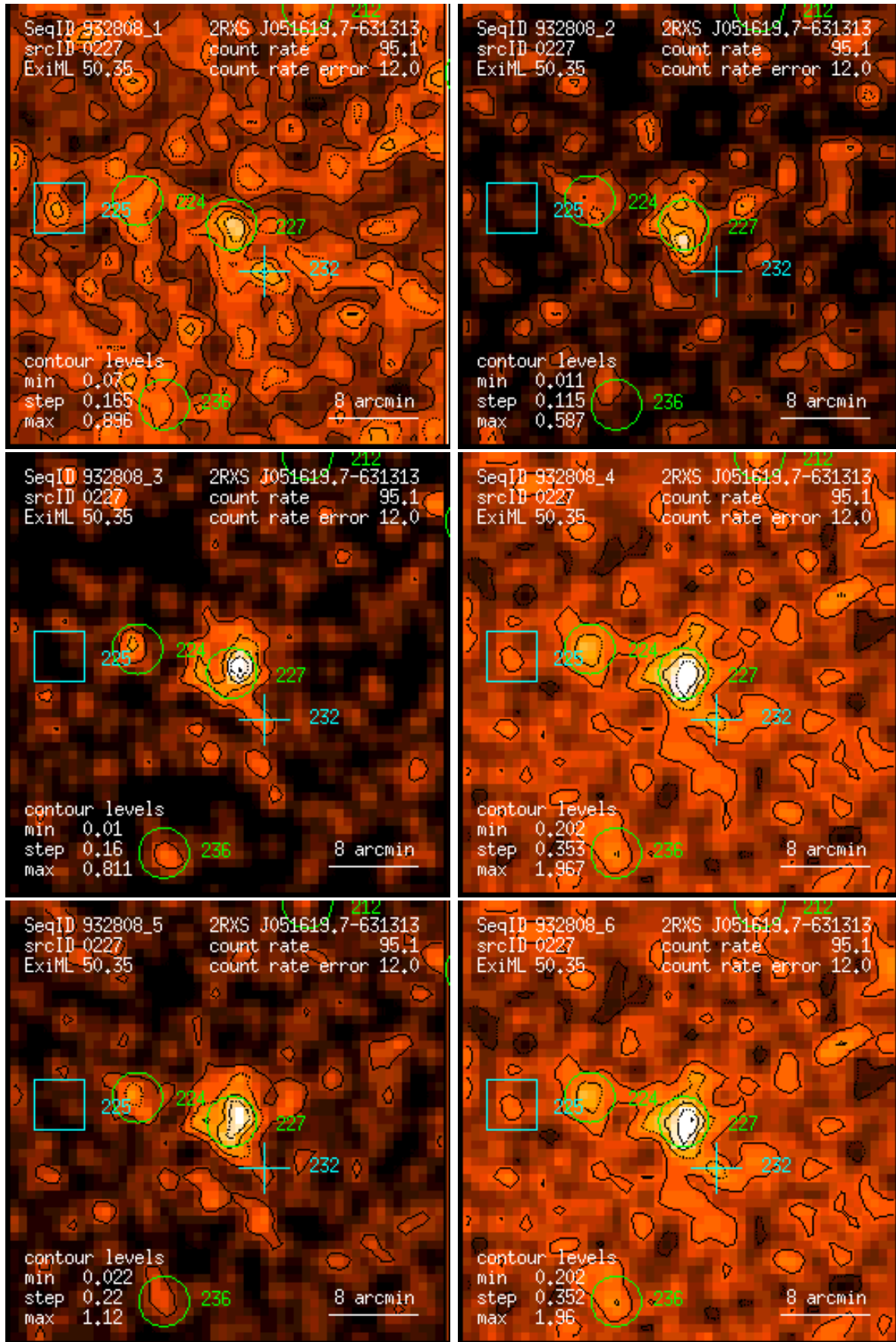
Figure 227: RASS 932808: detection 0227: band rate images, Gaussian filter: (1) PSPC channels 11 – 41, (2) 52 – 90, (3) 91 – 201, (4) 11 – 235, (5) 52 – 201, (6) 11 – 201. Broad band rates in counts/ks. Band rate contour levels in counts/ks/arcmin 2 .
