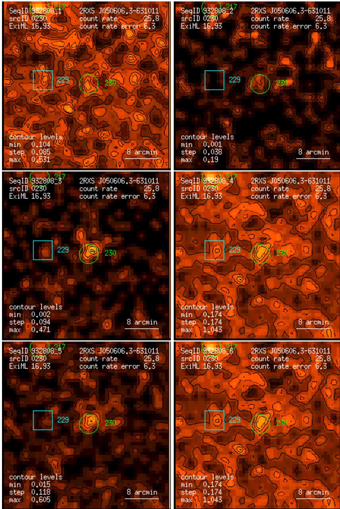
Figure 230: RASS 932808: detection 0230: band rate images, Gaussian filter: (1) PSPC channels 11 – 41, (2) 52 – 90, (3) 91 – 201, (4) 11 – 235, (5) 52 – 201, (6) 11 – 201. Broad band rates in counts/ks. Band rate contour levels in counts/ks/arcmin 2 .
