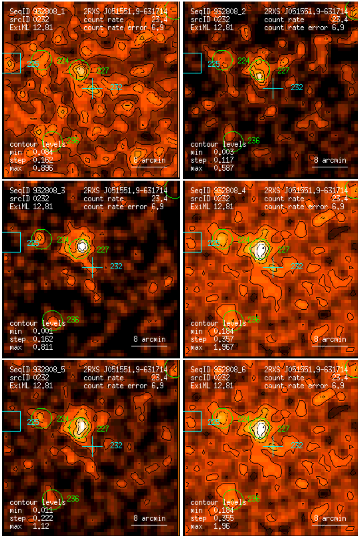
Figure 232: RASS 932808: detection 0232: band rate images, Gaussian filter: (1) PSPC channels 11 – 41, (2) 52 – 90, (3) 91 – 201, (4) 11 – 235, (5) 52 – 201, (6) 11 – 201. Broad band rates in counts/ks. Band rate contour levels in counts/ks/arcmin 2 .
