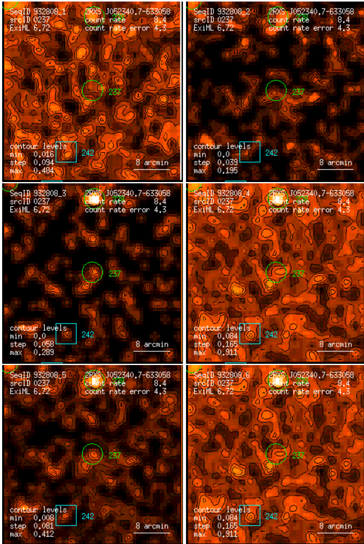
Figure 237: RASS 932808: detection 0237: band rate images, Gaussian filter: (1) PSPC channels 11 – 41, (2) 52 – 90, (3) 91 – 201, (4) 11 – 235, (5) 52 – 201, (6) 11 – 201. Broad band rates in counts/ks. Band rate contour levels in counts/ks/arcmin 2 .
