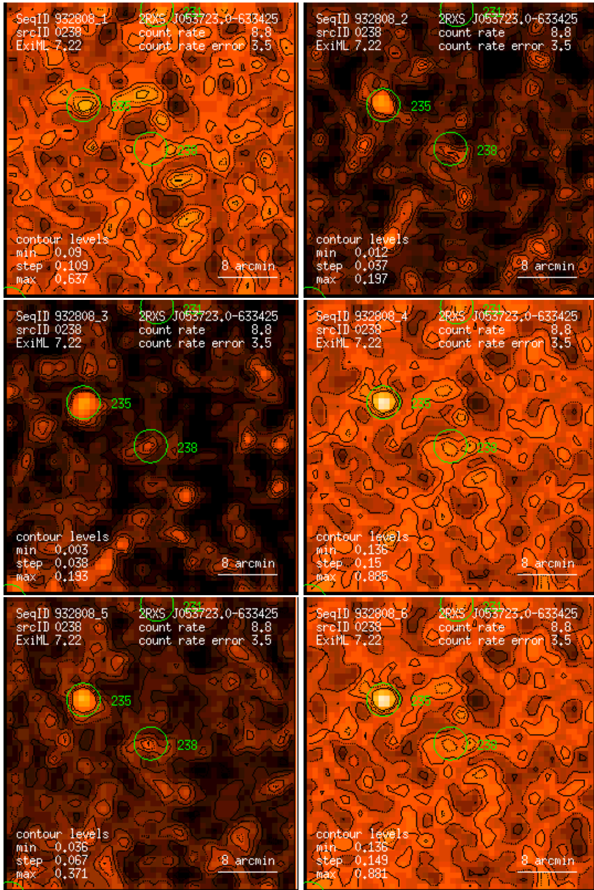
Figure 238: RASS 932808: detection 0238: band rate images, Gaussian filter: (1) PSPC channels 11 – 41, (2) 52 – 90, (3) 91 – 201, (4) 11 – 235, (5) 52 – 201, (6) 11 – 201. Broad band rates in counts/ks. Band rate contour levels in counts/ks/arcmin 2 .
