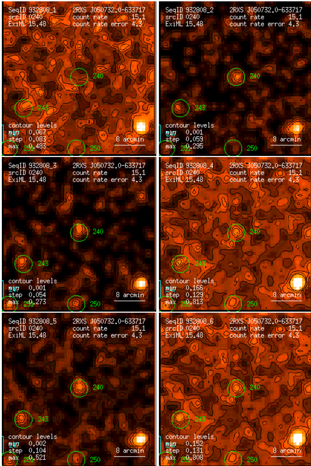
Figure 240: RASS 932808: detection 0240: band rate images, Gaussian filter: (1) PSPC channels 11 – 41, (2) 52 – 90, (3) 91 – 201, (4) 11 – 235, (5) 52 – 201, (6) 11 – 201. Broad band rates in counts/ks. Band rate contour levels in counts/ks/arcmin 2 .
