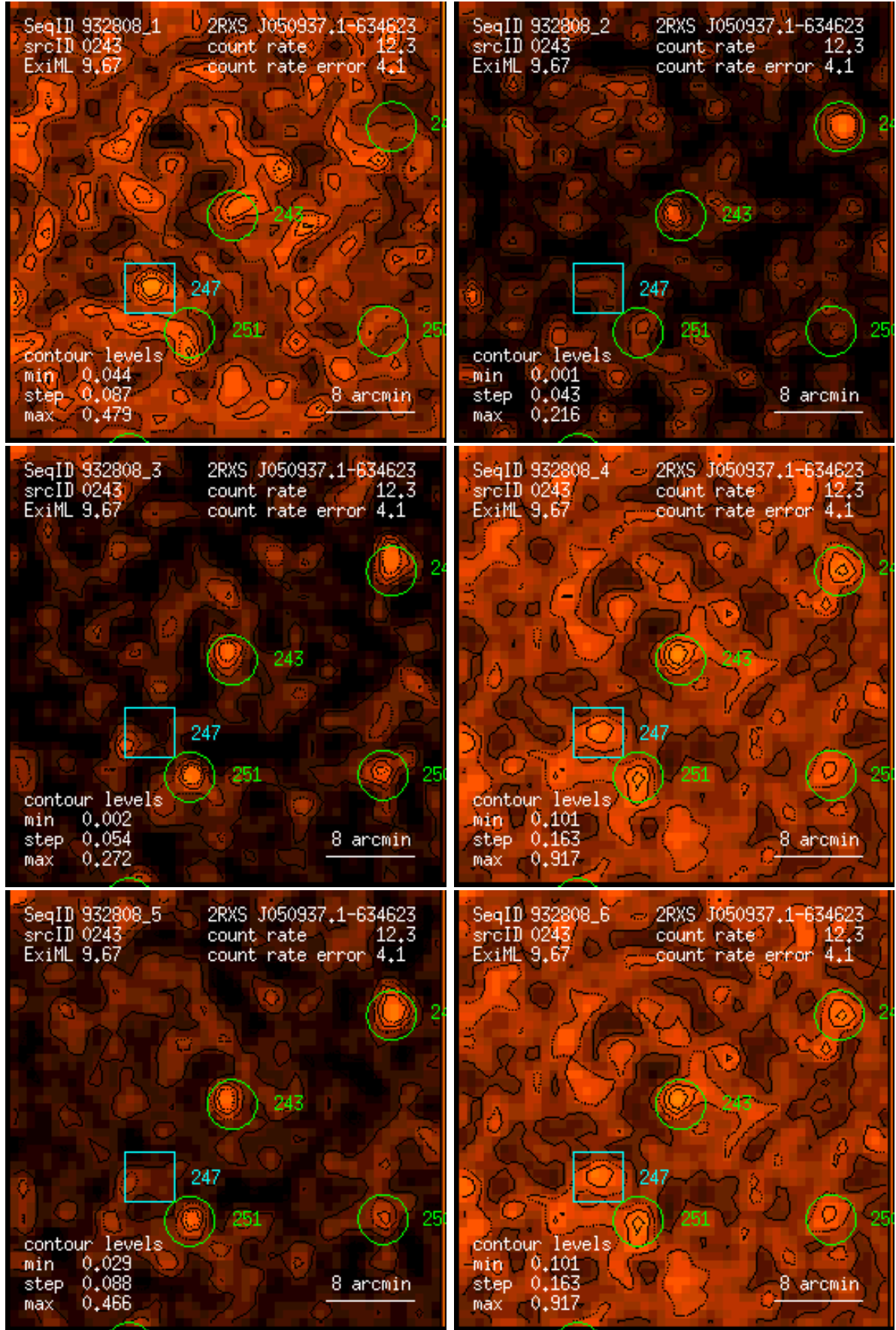
Figure 243: RASS 932808: detection 0243: band rate images, Gaussian filter: (1) PSPC channels 11 – 41, (2) 52 – 90, (3) 91 – 201, (4) 11 – 235, (5) 52 – 201, (6) 11 – 201. Broad band rates in counts/ks. Band rate contour levels in counts/ks/arcmin 2 .
