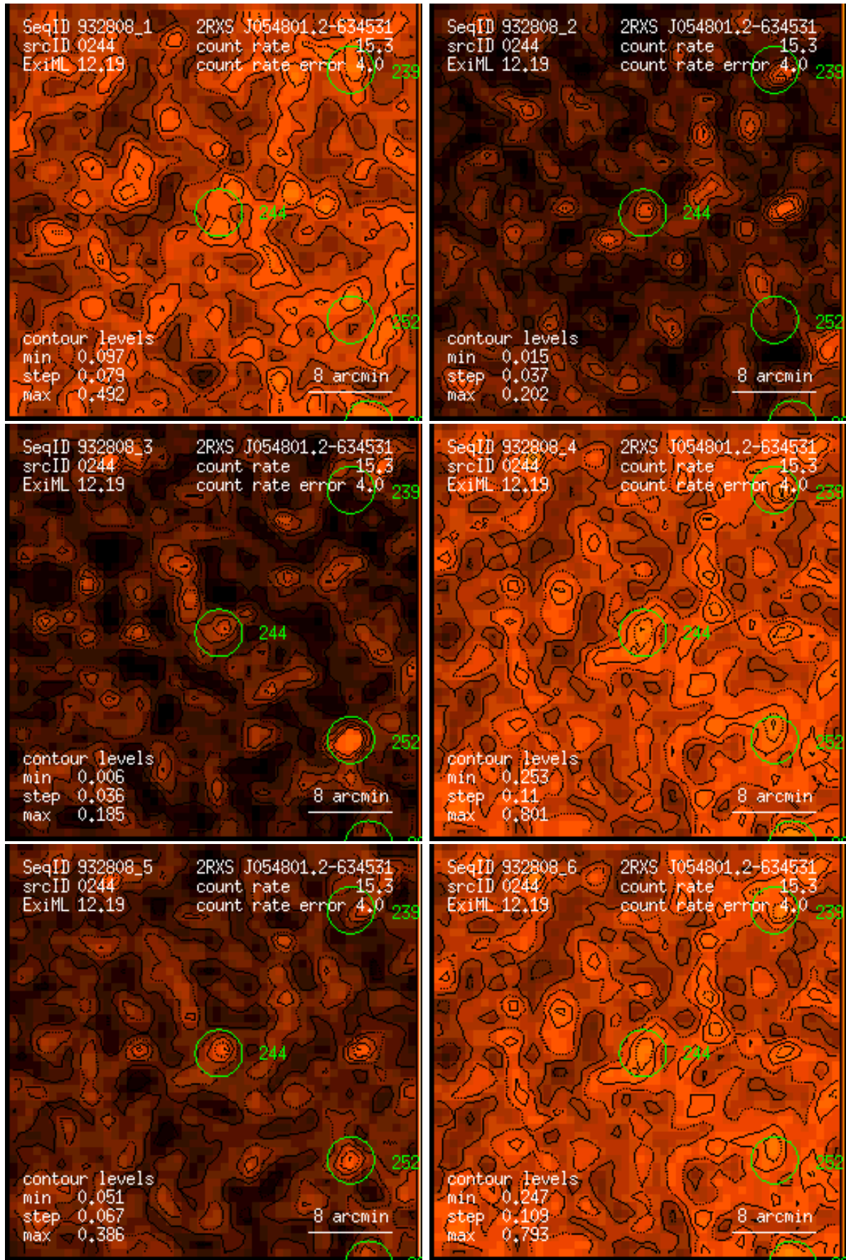
Figure 244: RASS 932808: detection 0244: band rate images, Gaussian filter: (1) PSPC channels 11 – 41, (2) 52 – 90, (3) 91 – 201, (4) 11 – 235, (5) 52 – 201, (6) 11 – 201. Broad band rates in counts/ks. Band rate contour levels in counts/ks/arcmin 2 .
