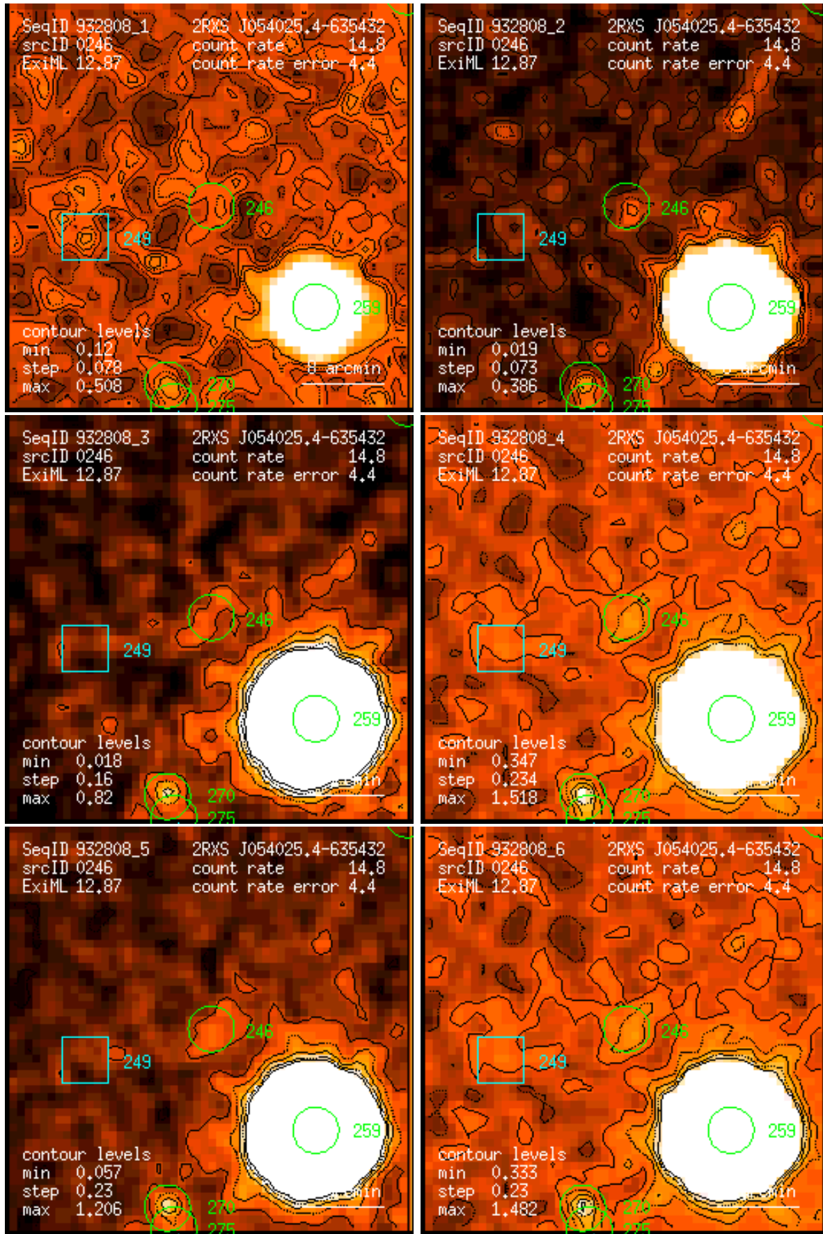
Figure 246: RASS 932808: detection 0246: band rate images, Gaussian filter: (1) PSPC channels 11 – 41, (2) 52 – 90, (3) 91 – 201, (4) 11 – 235, (5) 52 – 201, (6) 11 – 201. Broad band rates in counts/ks. Band rate contour levels in counts/ks/arcmin 2 .
