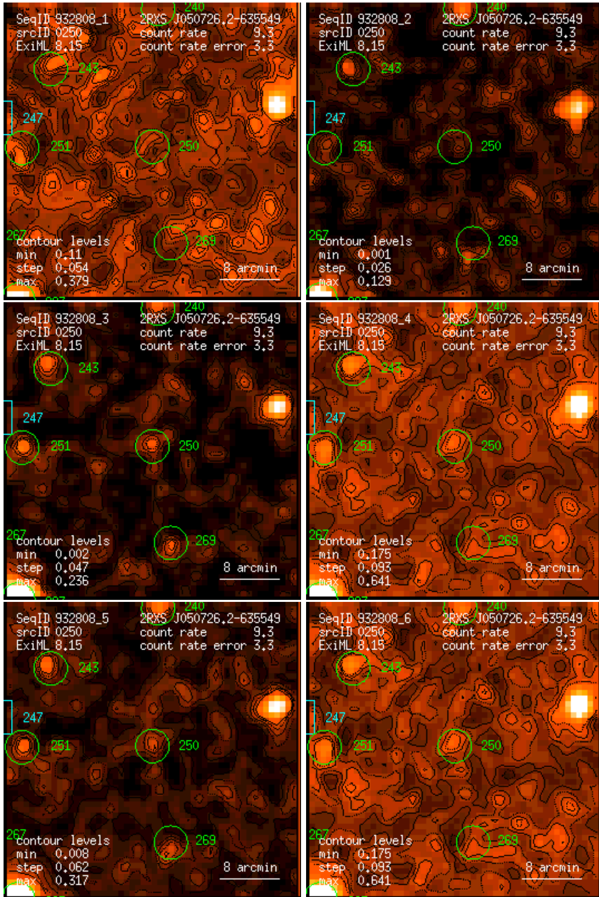
Figure 250: RASS 932808: detection 0250: band rate images, Gaussian filter: (1) PSPC channels 11 – 41, (2) 52 – 90, (3) 91 – 201, (4) 11 – 235, (5) 52 – 201, (6) 11 – 201. Broad band rates in counts/ks. Band rate contour levels in counts/ks/arcmin 2 .
