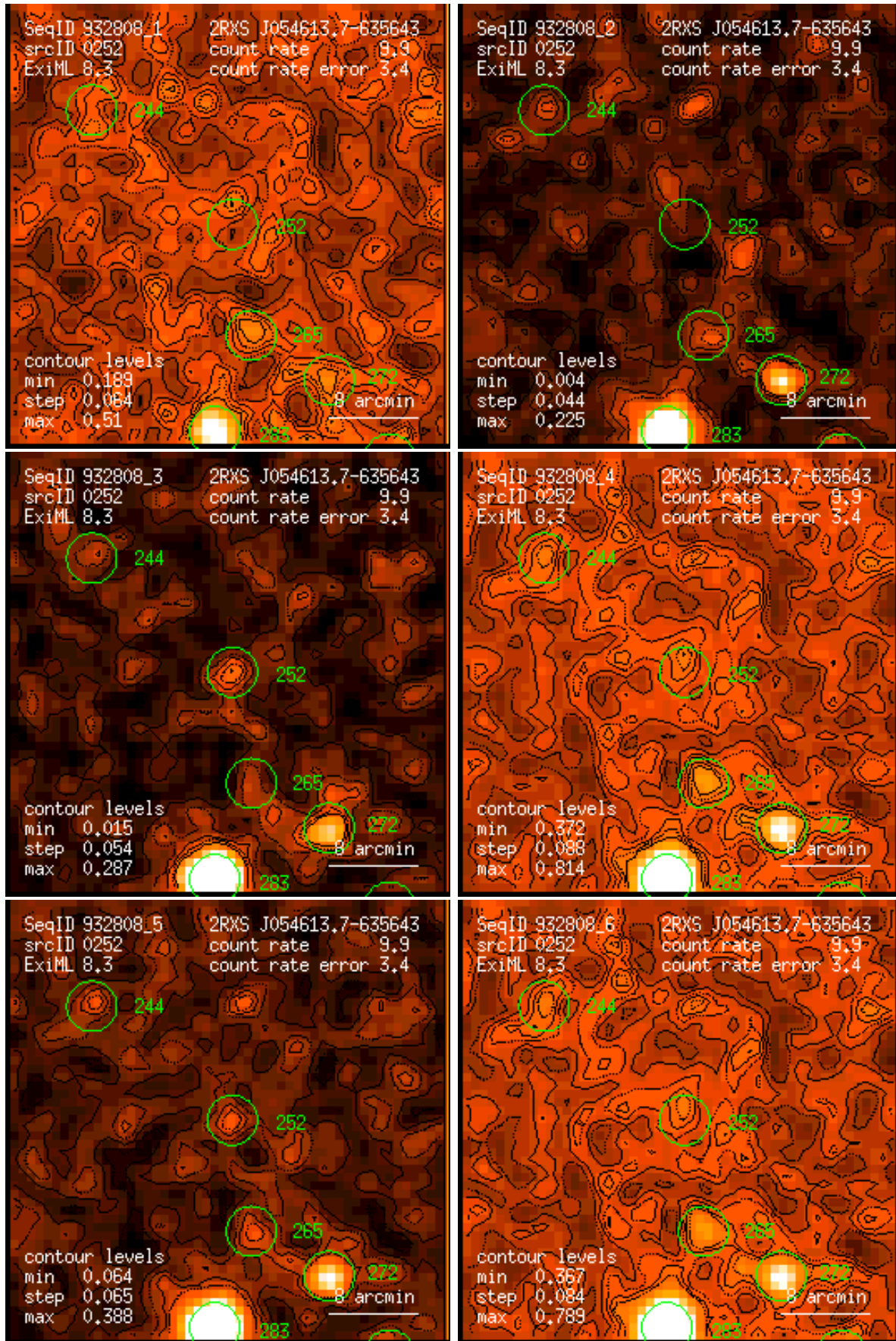
Figure 252: RASS 932808: detection 0252: band rate images, Gaussian filter: (1) PSPC channels 11 – 41, (2) 52 – 90, (3) 91 – 201, (4) 11 – 235, (5) 52 – 201, (6) 11 – 201. Broad band rates in counts/ks. Band rate contour levels in counts/ks/arcmin 2 .
